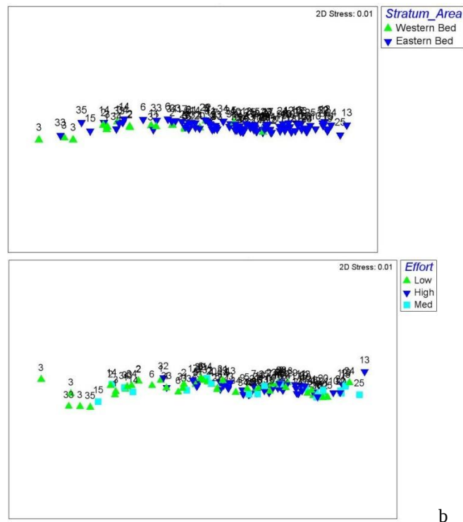
Figure 7.19. Multi-dimensional scaling (MDS) using the Bray Curtis resemblance to compare scallop abundance rankings a) across the two regions and b) between fished and non-fished sites at three levels of fishing effort.
