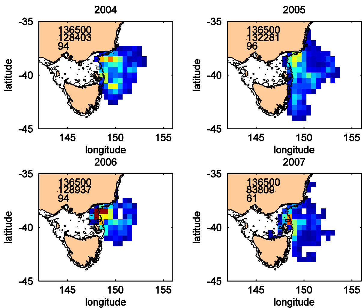
Figure 7.13. Aggregate compilation of the dispersal end point from all release days by year, from blue to red indicates a higher number of scallops in the \frac{1}{2} degree block.
