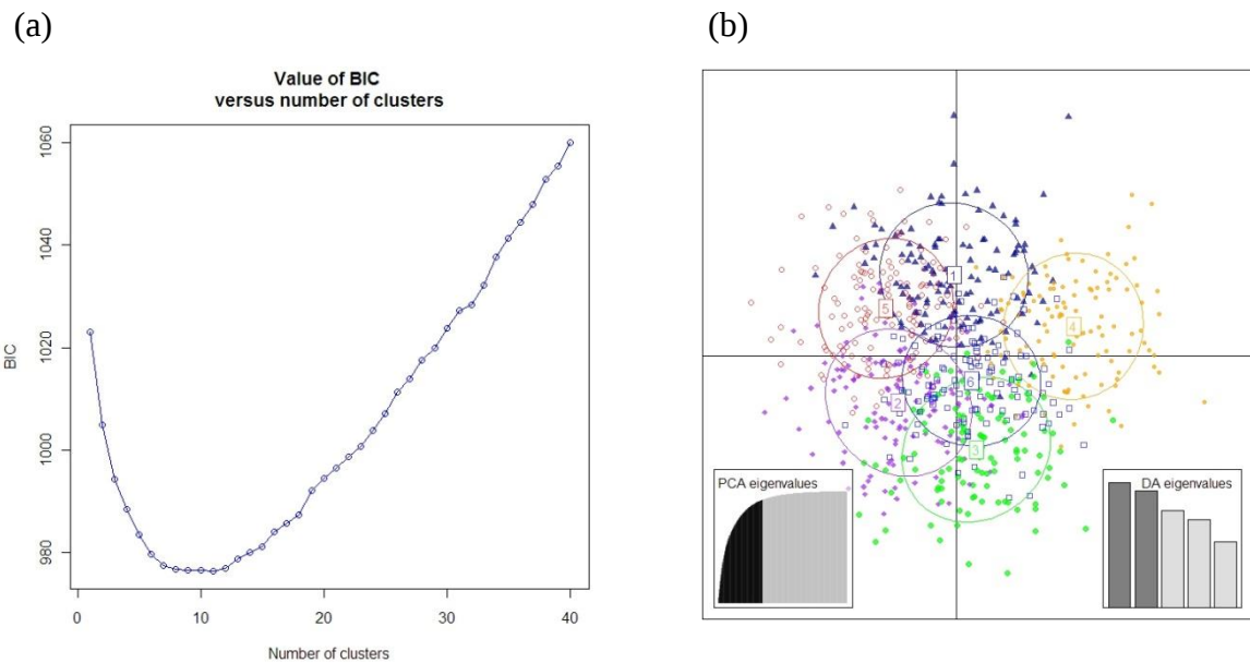
Figure 7.7. Discriminant analysis of principal components from a random genotype dataset generated from empirical allele frequencies (a) Bayesian Information Criterion (BIC) to assess the best supported model and (b) scatter plot of the first two principal components in a model with six clusters selected.
