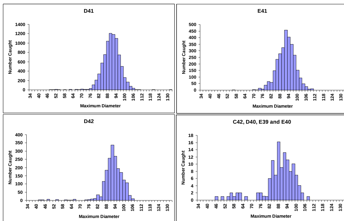
Figure 8: The length frequency distribution for scallops caught within grids D41, D42, E41 and grids C42, D40, E39 and E40 combined.
