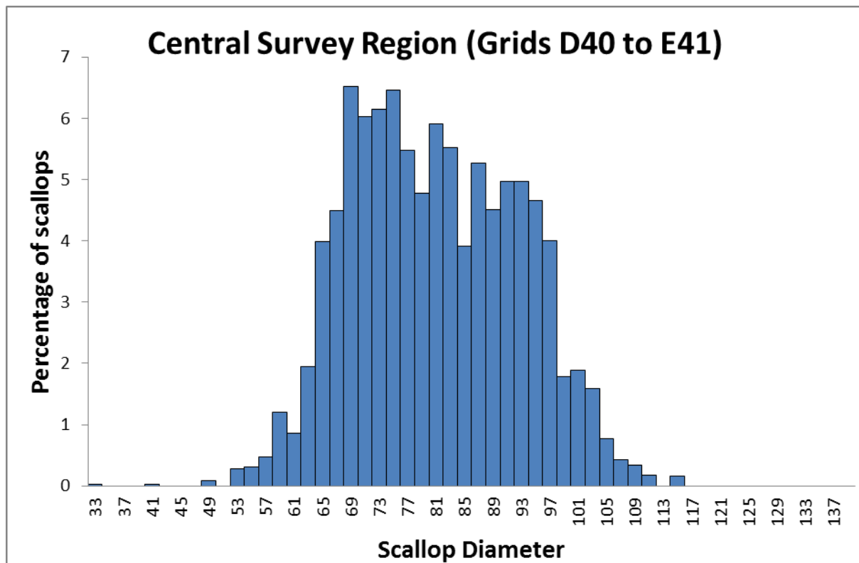
Figure 8: The length frequency distribution for scallops measured within grids D40 to E41. A total of 1259 scallops were measured in this region.
