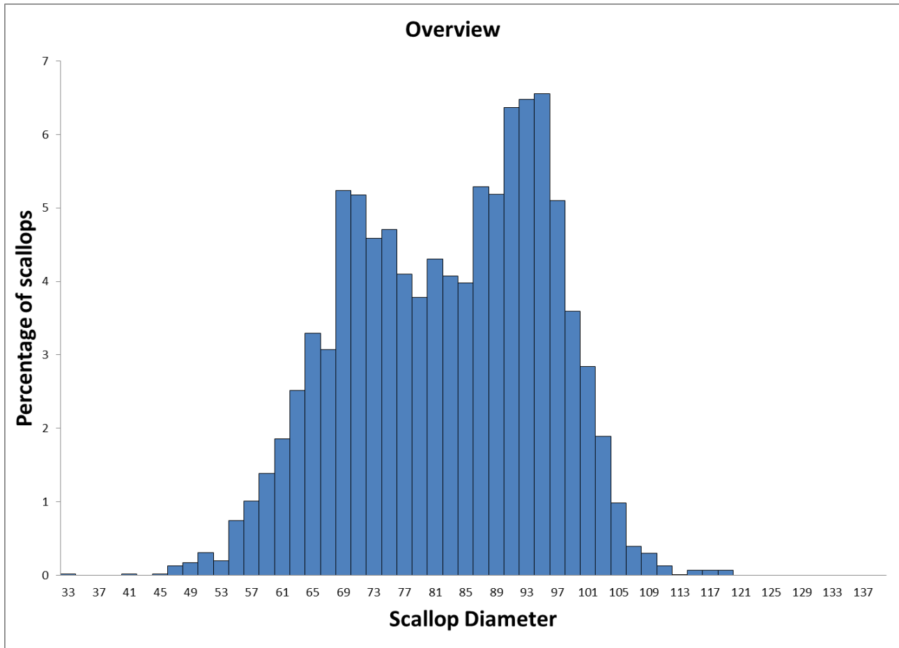
Figure 4: The length frequency distribution for all scallops measured during the 2012 survey
