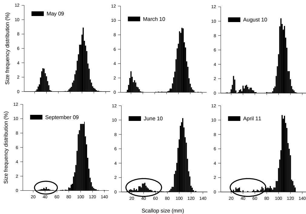
Figure 7.24. Length frequency distribution for scallops measured within the Great Bay sampling locations (32 sites) at each sampling period. Black circles show the reduced number of recruits that survived the post-settlement period.
