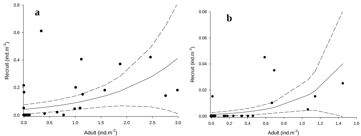
Figure 7.22. Relationship between adult and recruit density in a) 2010 and b) 2011. Black dots are the data points, continuous line indicates the model fit and dashed lines are the upper and lower 95% confidence intervals.
