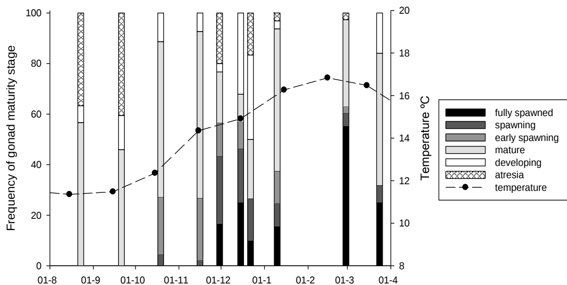
Figure 7.32. Relative frequency of gonad maturity stages in P. fumatus between August 2010 and March 2011 and monthly average temperature.
