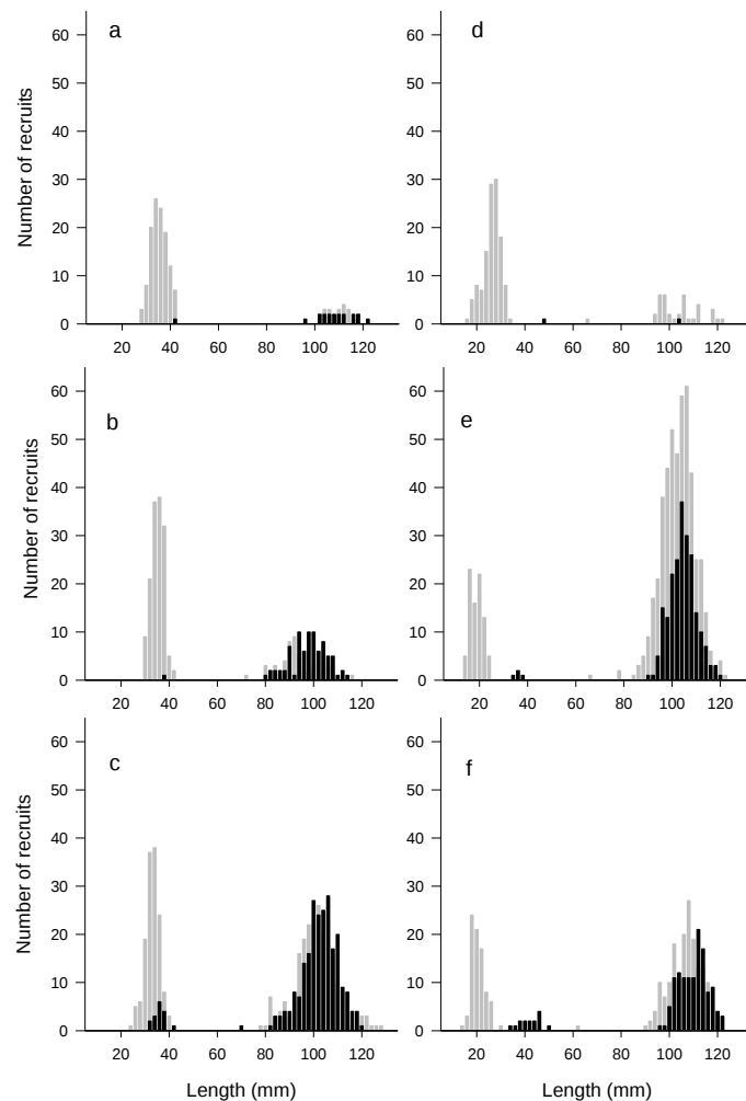
Figure 7.25. Length frequency distribution for scallops in three sites with strongest recruitment pulse in 2009 (a-c) in May (grey bars) and September (black bars) and in 2010 (d-f) in March (grey bars) and August 2010 (black bars).
