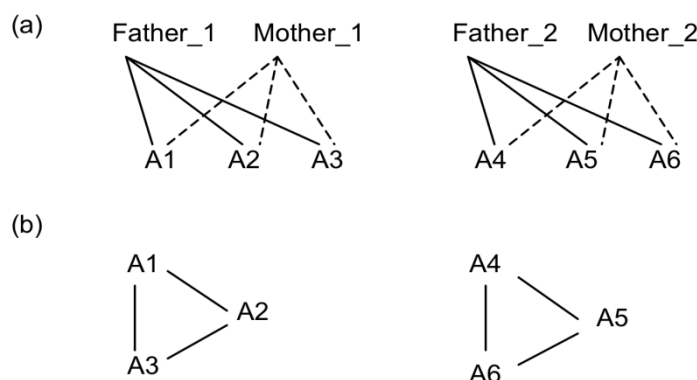
Figure 6.2. Control pedigree of six offspring (A1, A2, A3, A4, A5, A6) showing (a) 12 parent offspring (PO) relationships and (b) six full-sib (FS) relationships.
