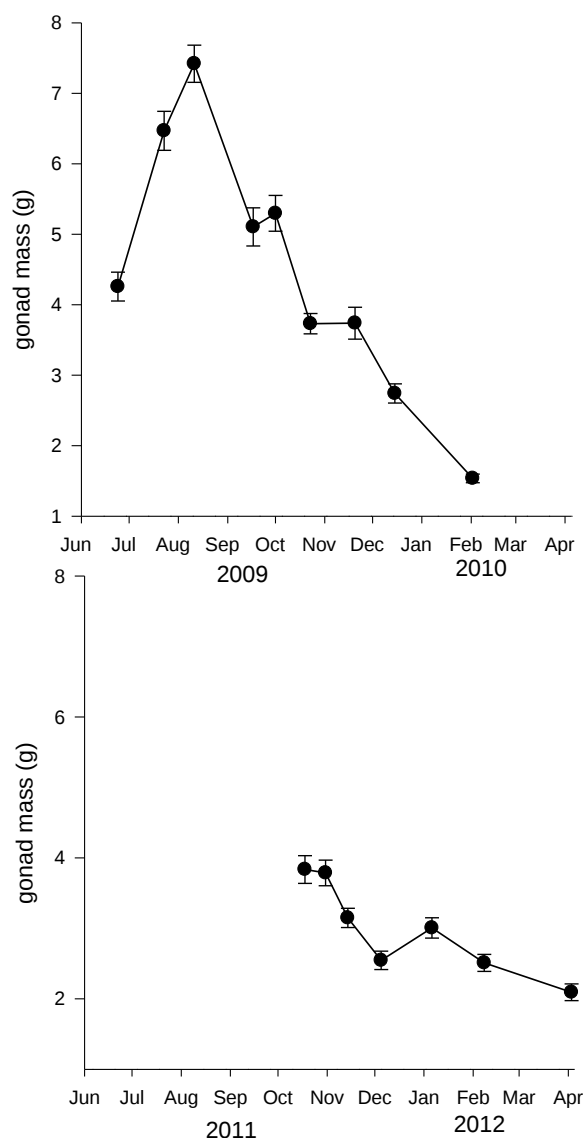
Figure 7.27. Gonadal mass for a standard scallop measuring 105 mm for a) spawning season 2009-10 and b) season 2010-11.
