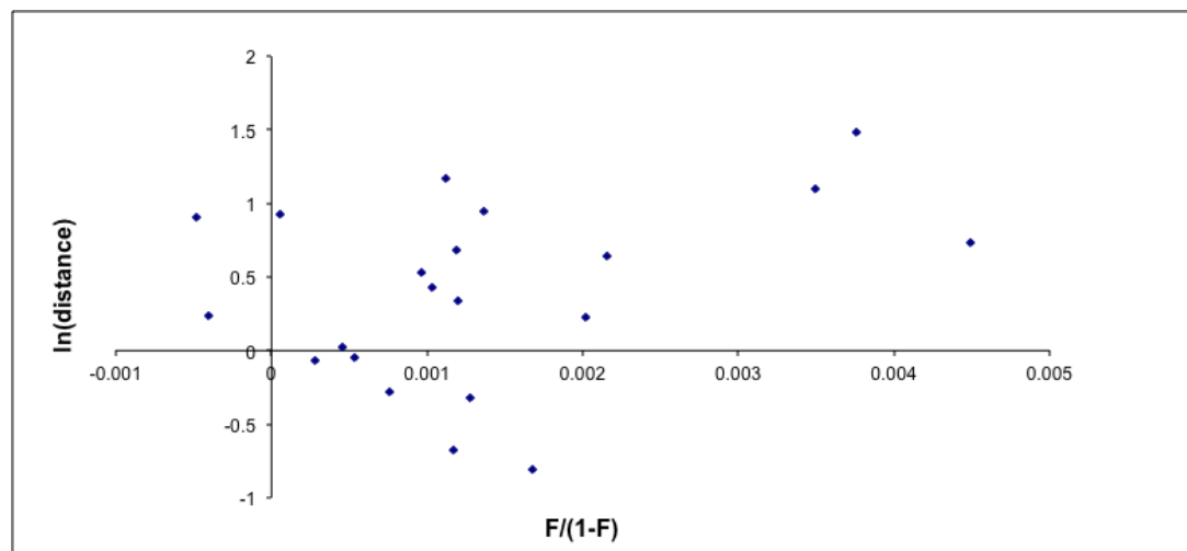
Figure 7.2. A plot of genetic distance ( F_{ST} / (1 - F_{ST}) ) compared to geographic distance (ln km) for seven regional sampling locations in open waters (i.e. without embayment locations of Port Phillip Bay and D'Entrecasteaux Channel, DEC) of P. fumatus at 11 microsatellite loci. Mantel test for isolation by distance was insignificant ( p < 0.256 ).
