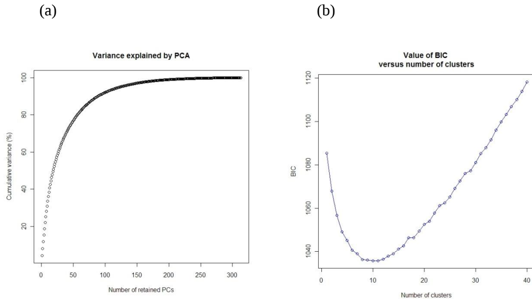
Figure 7.5. Analysis of P. fumatus genotypes with 11 loci (D2.dat, table 6.1): (a) variance explained by number of retained principal components (PSs) and (b) Bayesian Information Criterion (BIC) to assess the best supported model i.e. the number of clusters in the eleven locus dataset.
