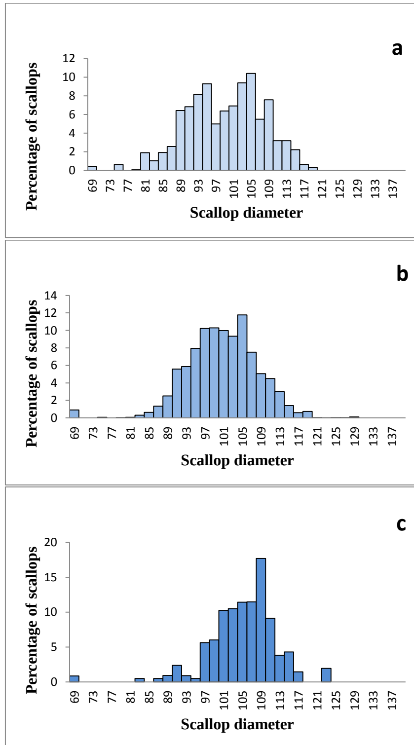
Figure 7.20. Comparison of size frequencies for scallops caught during the 2010 post fishing season survey from sites that were: (a) never fished n = 233; (b) fished for a single year, during the 2010 season (note that all sites that were fished in 2009 were also fished in 2010) n = 1767; and (c), fished in both 2009 and 2010 n = 211.
