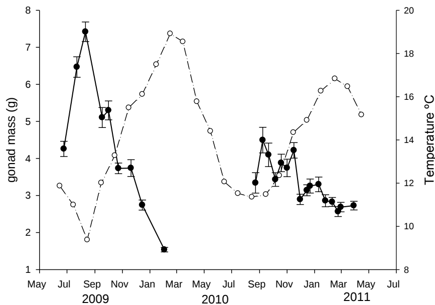
Figure 7.28. Gonad mass index (black dots) and average monthly sea surface temperature (white dots) estimated from MODISA satellite data.
