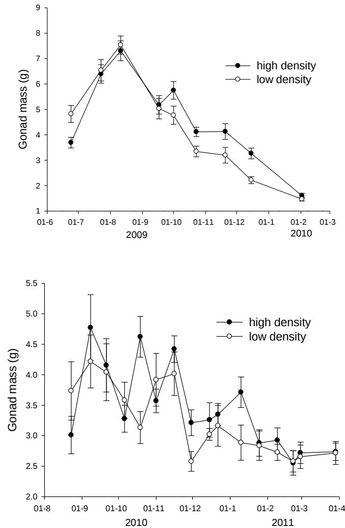
Figure 7.29. Gonad mass for high density and low density areas during spawning season 2009-10 a) and 2010-11b).
