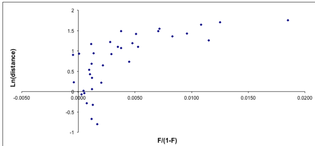
Figure 7.1. A plot of genetic distance ( F_{ST} / (1 - F_{ST}) ) and geographic distance (ln km) for nine regional sampling locations of P. fumatus at 11 microsatellite loci. Mantel test for isolation by distance was significant ( p < 0.00087 ).
