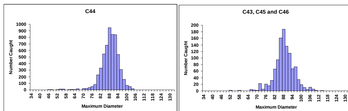
Figure 10: The length frequency distribution for scallops caught within grids C44 and grids C43, C45 and C46 combined.
