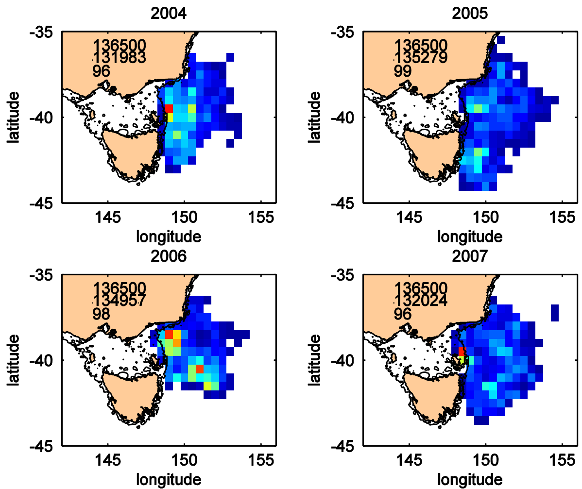
Figure 7.9. Aggregate compilation of the dispersal end point from all release days by year, from blue to red indicates a higher number of scallops in the \frac{1}{2} degree block.
