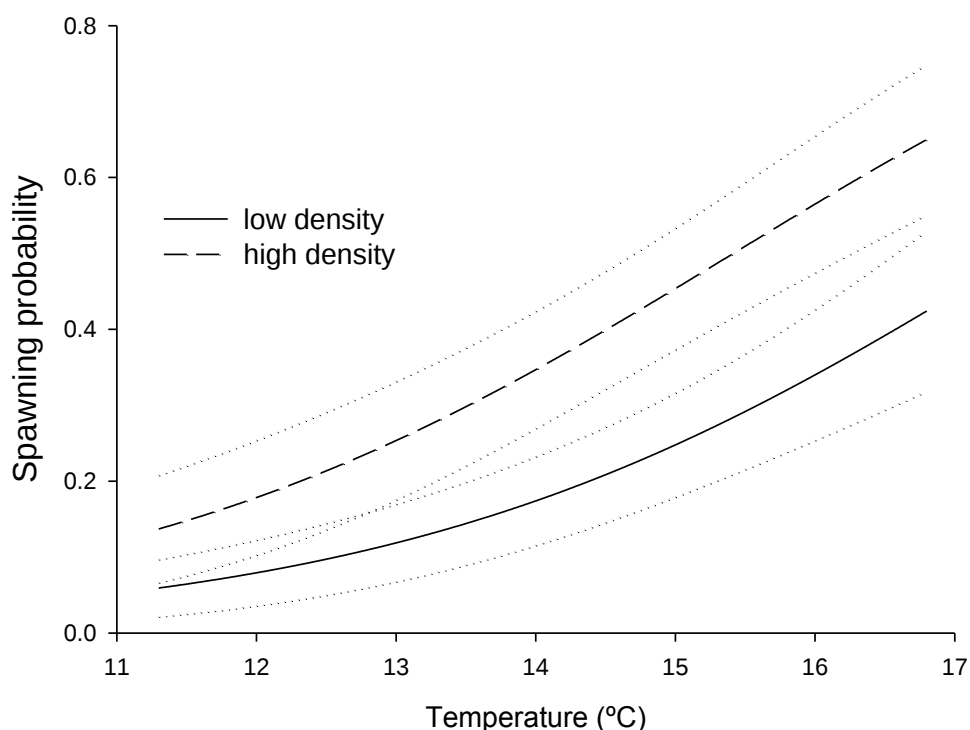
Figure 7.34. Spawning probabilities at different temperatures in a high density and low density site. Dash lines represent the model for high density and continuous line is the model for low density.
