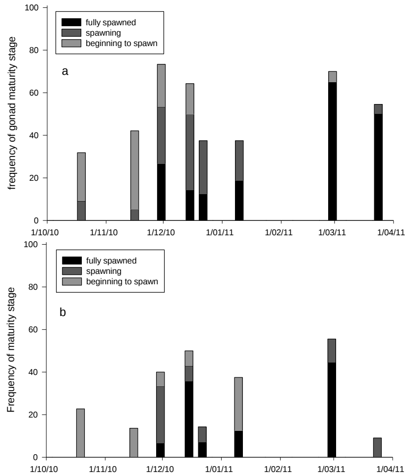
Figure 7.33. Relative frequencies of spawning stages (beginning to spawn, spawning and fully spawned) in a) high and b) low density areas from October 2010 to March 2011.
