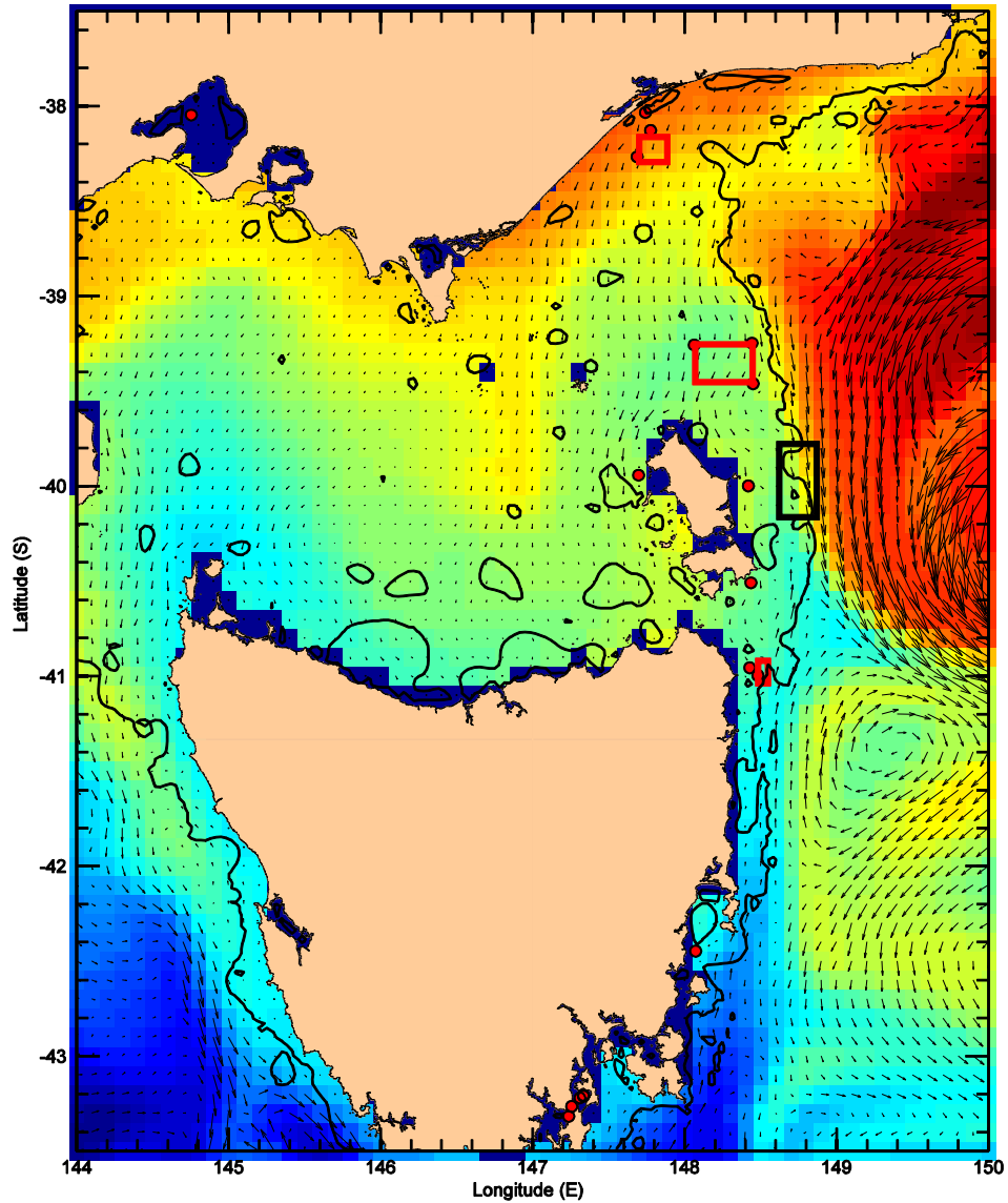
Figure 6.3. The current fields and water temperature (at 10-20 m depth) from the BRAN 2.1 model are shown. The dark blue areas close to the coast indicate areas outside the domain of the BRAN product i.e. no data. The black box east of Flinders Island represents the spawning box from which the 30 spawning nodes were randomly dispersed for the first run of the model. The red dots indicate where scallop samples were collected in 2008/09. The red spawning boxes indicate the position of other spawning boxes from which spawning nodes were randomly dispersed.
