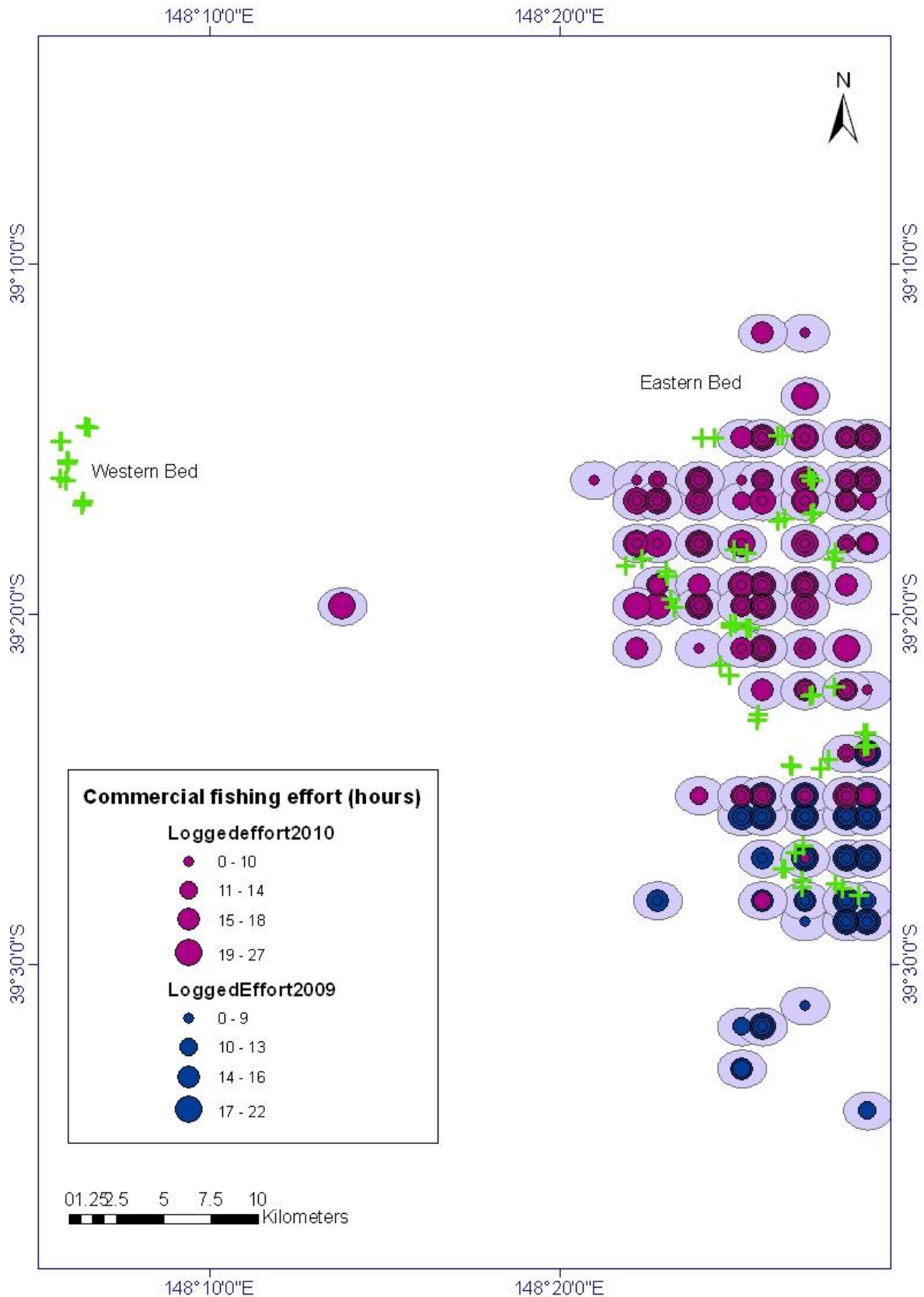
Figure 6.6. Survey dredge shots (crosses) that fell within areas of specific fishing effort in 2009 (blue) and 2010 (purple), according to average length of a standard trawl ~500m. Fishing effort, in hours fished, was overlaid on the map as an area of 1 km in diameter around logged dredge start locations.
