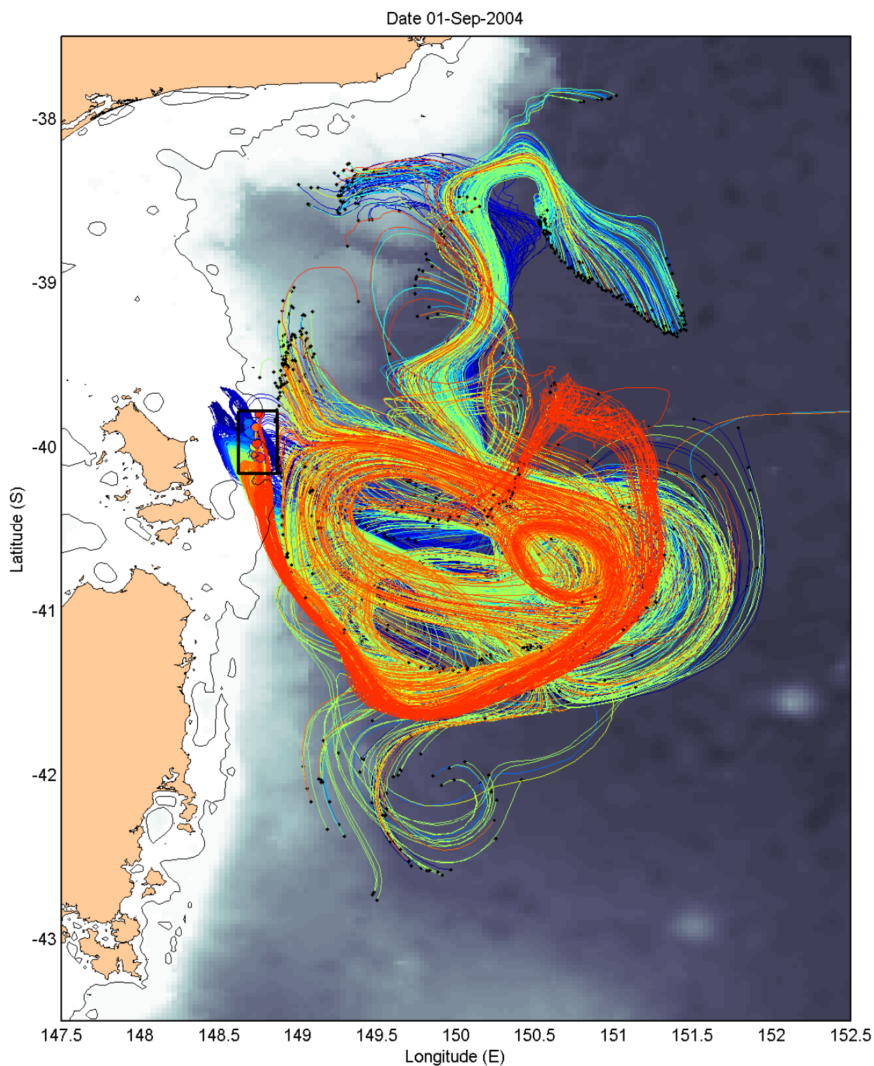
Figure 7.8. An example showing the spawning nodes (coloured circles within black box), dispersal trajectories (coloured lines corresponding to spawning node colours) and end points (black points) from 10 of the 30 spawning nodes off East Flinders Island.
