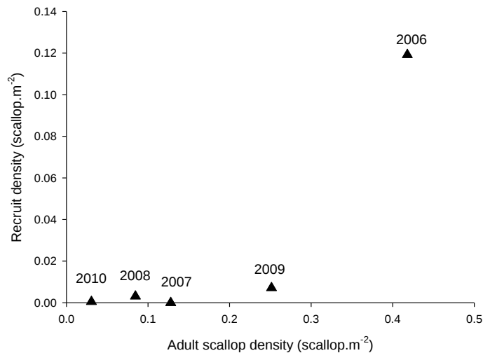
Figure 7.26. Relationship between density of adults and density of recruits in 24 sites throughout the DEC from 2006-2010.
