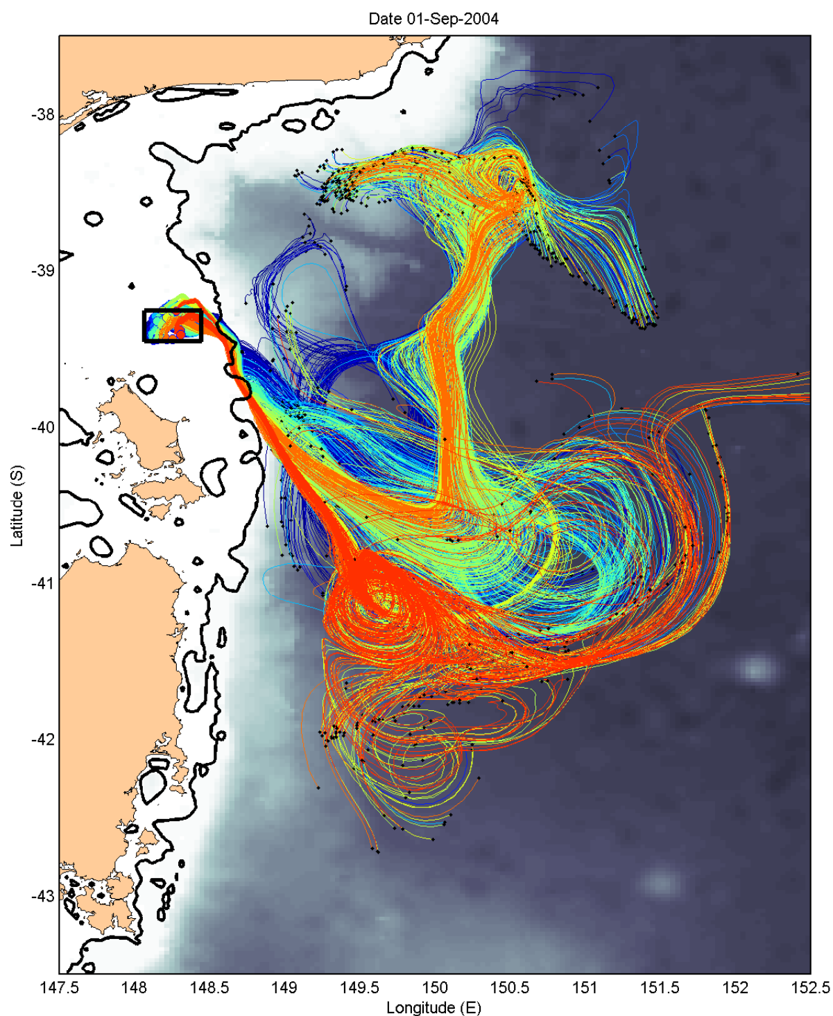
Figure 7.12. An example showing the spawning nodes (coloured circles within black box), dispersal trajectories (coloured lines corresponding to spawning node colours) and end points (black points) from 10 of the 30 spawning nodes in the Commonwealth BSCZ.
