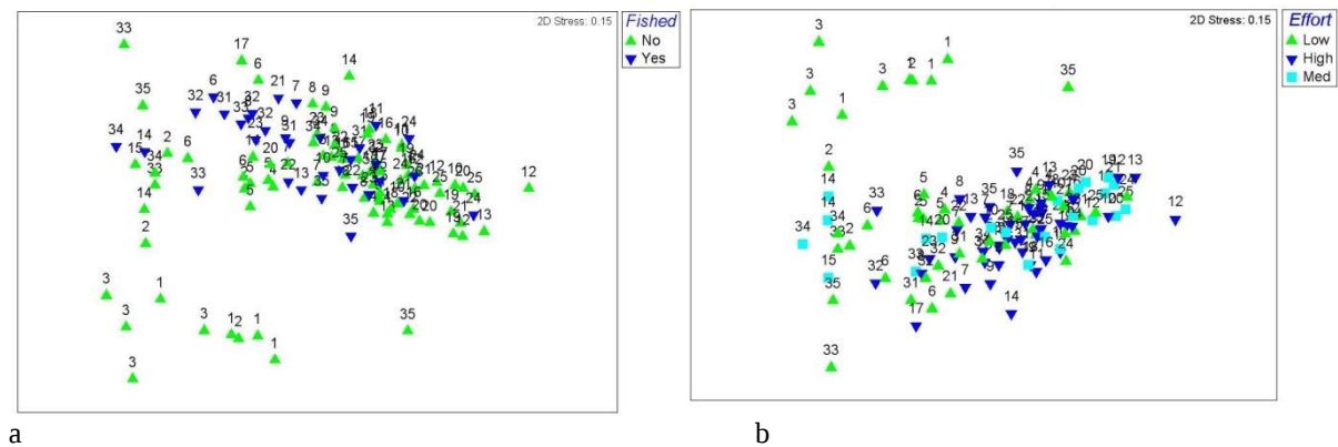
Figure 7.17. a): Multi-dimensional scaling (MDS) using the Bray Curtis resemblance to compare species abundance rankings between a) survey sites that were fished (blue inverted triangles) and control (green triangles) sites and b) survey sites located in areas of different levels of fishing pressure. Survey sites are numbered, with 1- 6 belonging to the western bed and the rest to the Eastern region (multiple numbers are due to multiple surveys).
