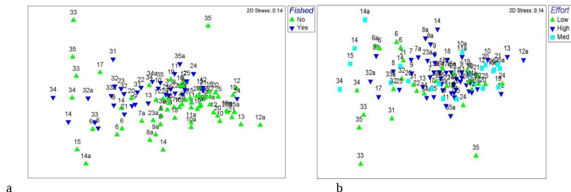
Figure 7.18. MDS ranking of sites within the eastern region only at levels of a) fished or control, and b) three levels of fishing effort.
