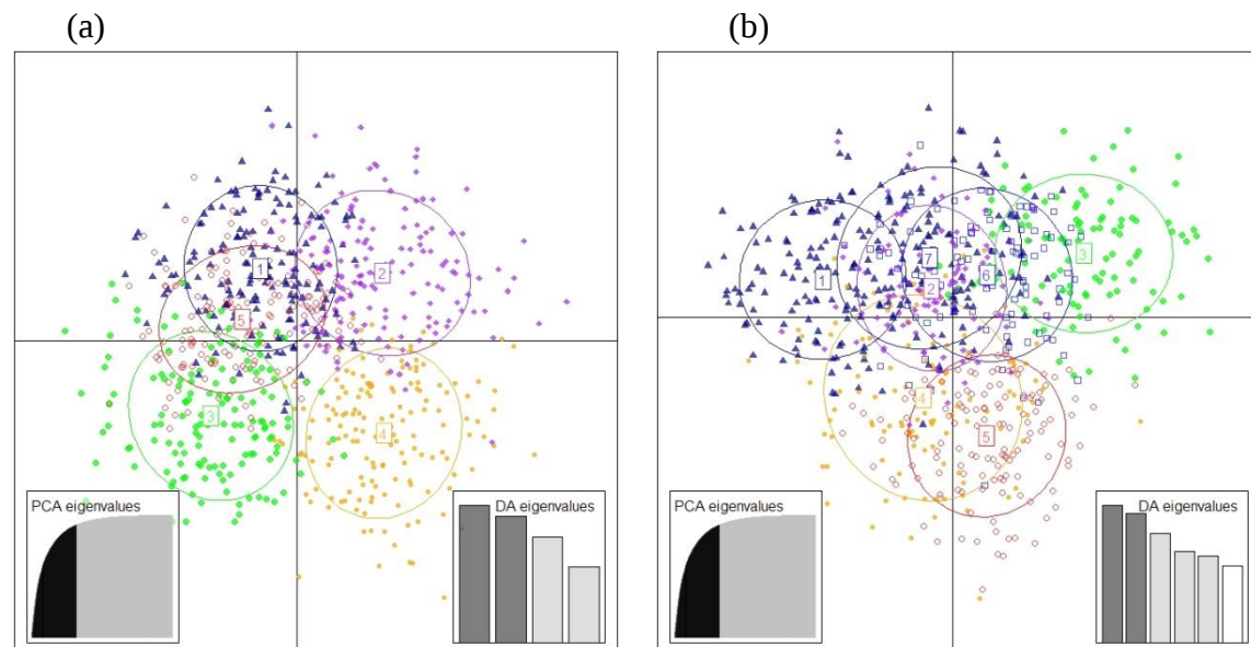
Figure 7.6. Analysis of P. fumatus genotypes with 11 loci (D2.dat, table 6.1): Plot of first and second principal components with (a) five clusters and (b) seven clusters.
