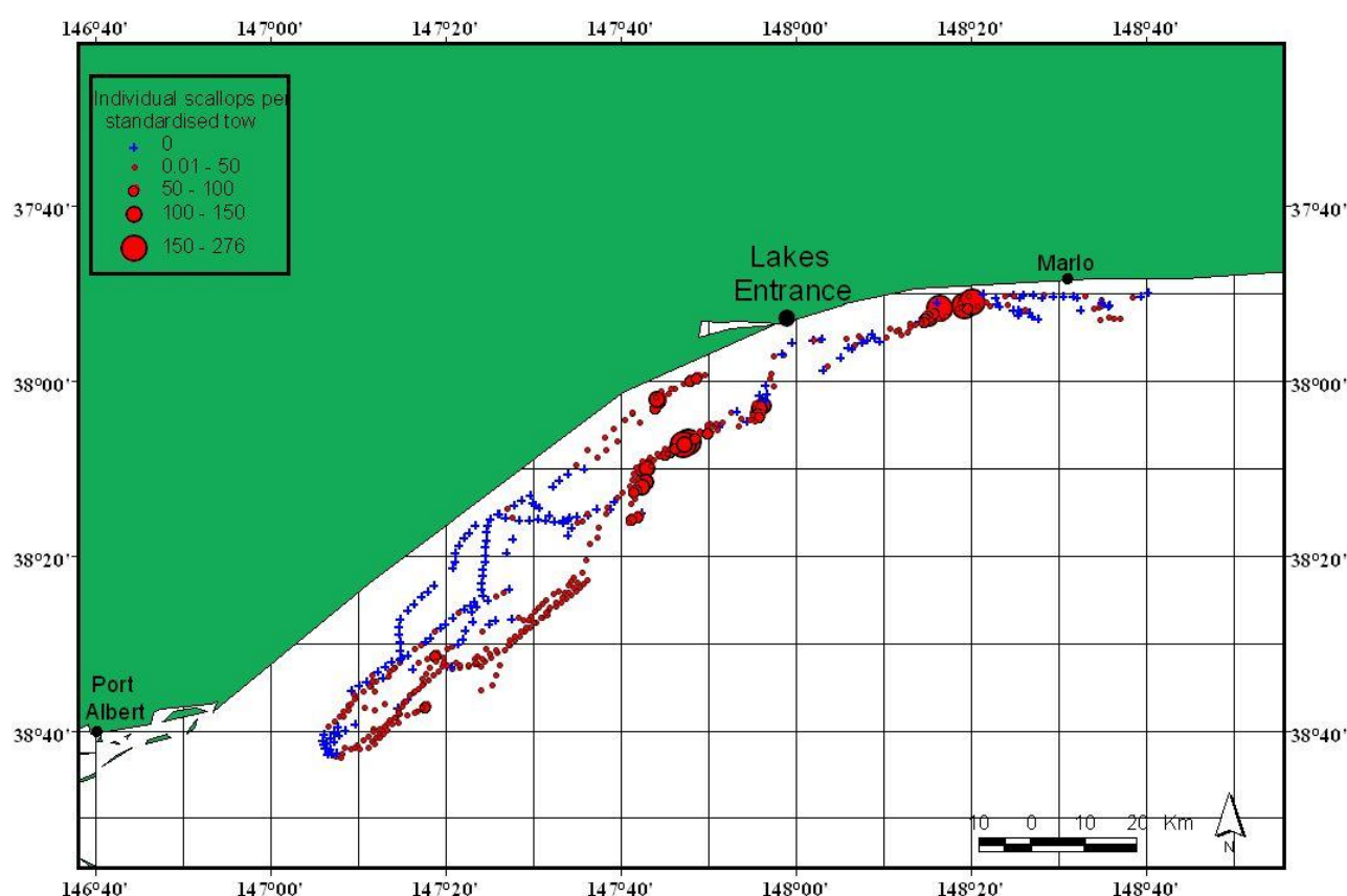
Figure 4: Scallop abundances (individual scallops per 1000m 2 sample tow) for tows conducted during the December 2009 Victorian scallop survey. The 10' latitude x 10' longitude grid is shown as a reference for later results.
