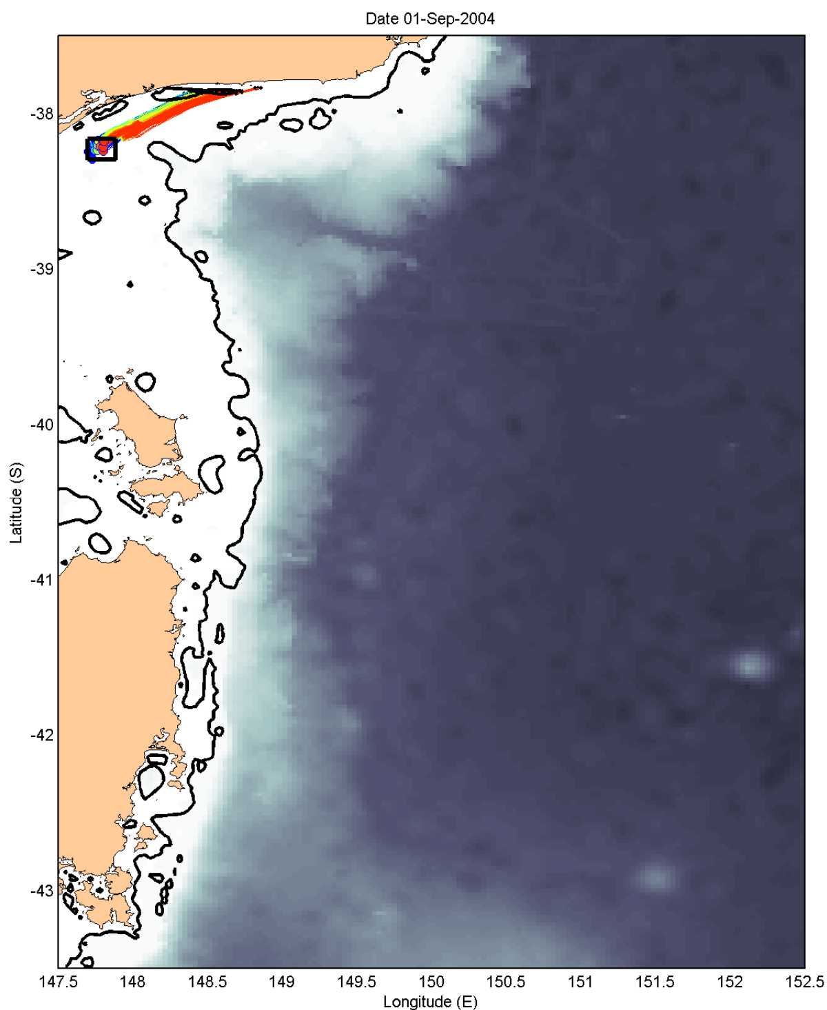
Figure 7.10. An example showing the spawning nodes (coloured circles within black box), dispersal trajectories (coloured lines corresponding to spawning node colours) and end points (black points) from 10 of the 30 spawning nodes off Lakes Entrance.
