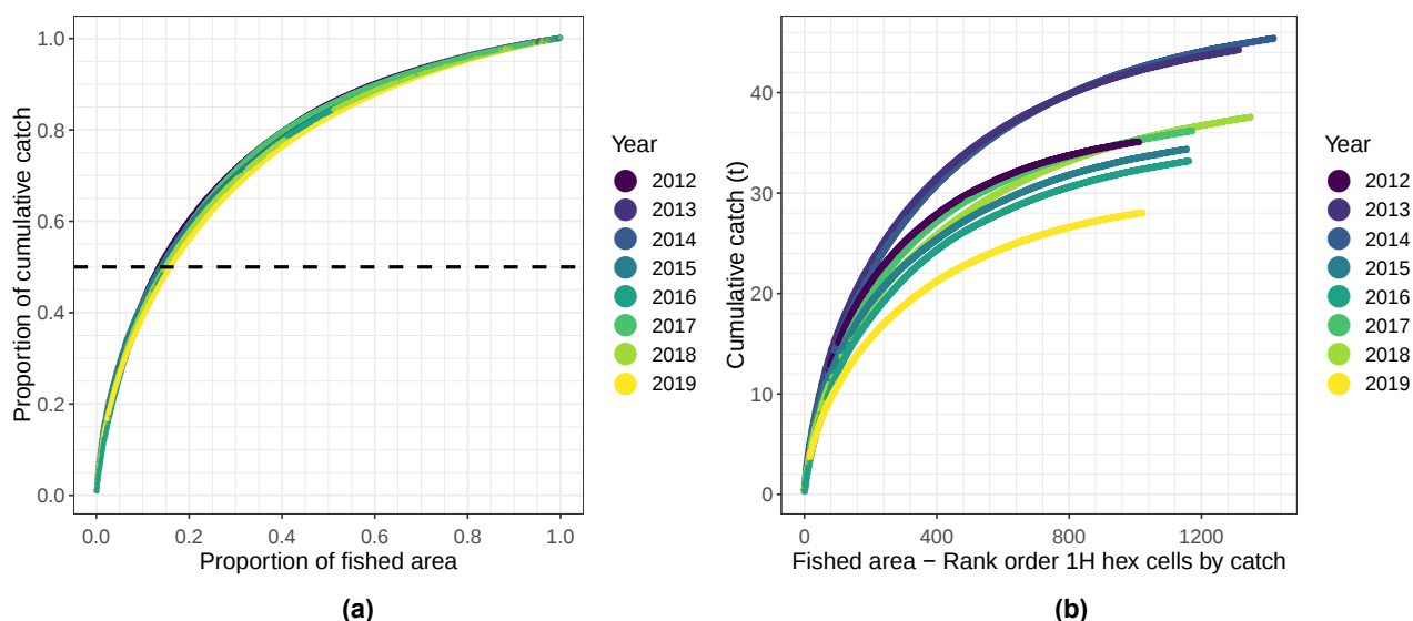
Figure 3.77: Concentration area curves for catch in the Greenlip Zone: a) Proportion of catch (y axis) against proportion of reef utilised (x axis). Hashed line represents 50% of catch; b) cumulative catch (y axis) against rank order of hex cells, descending from highest to smallest catch. Data filtered to exclude hex cells where less than 5 minutes of effort observed.
