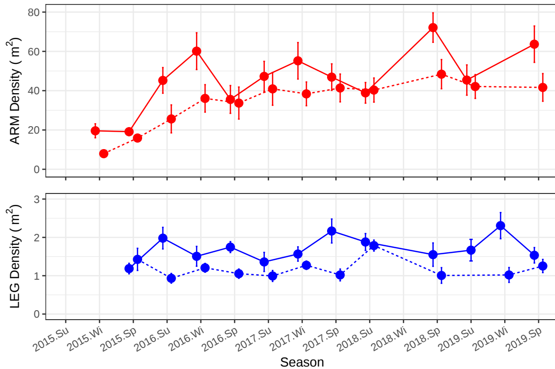
Figure 4.3: Mean density ( m^2 ) of abalone ( \pm SE) underneath ARMs (red) and recorded from LEG (blue) across the sampling period Summer 2015 to Spring 2019 at Black Reef Slab site (Block 14A). Each ARM has a planar surface area of 0.126m^2 . Replicate strings (sub-sites) are denoted by line type. Note the difference in density scale between the ARM and LEG results, and between ARM results of remaining sites.
