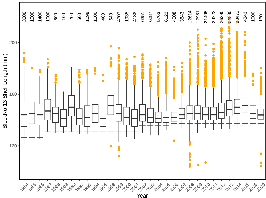
Figure 3.88: Boxplot of size distributions for Block 13 Eastern Zone between 1984 and 2019. Red line indicates legal minimum length for that year. Number of abalone measured given above each boxplot.
