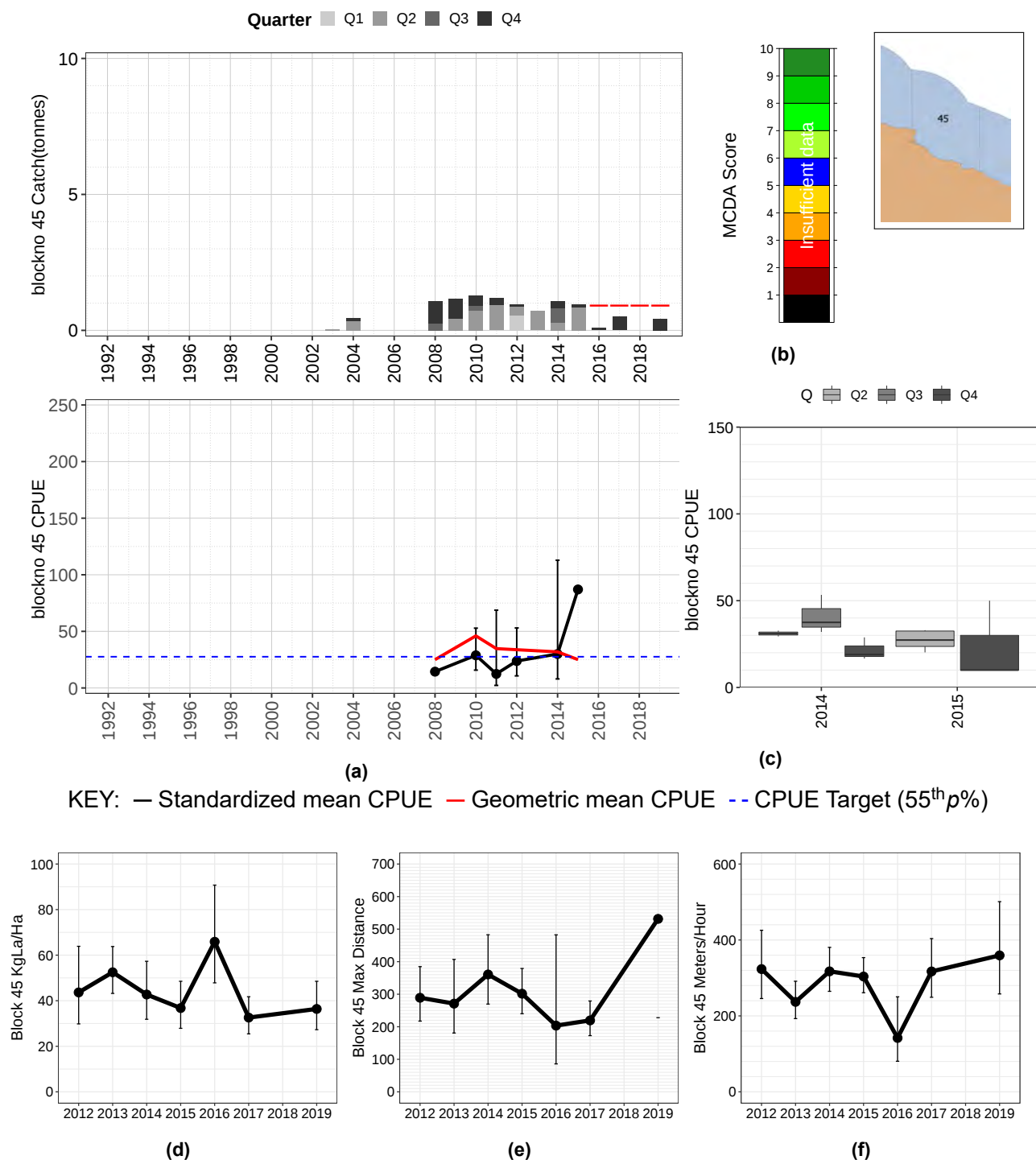
Figure 3.69: Block 45 BSZ: a) Catch per quarter (bars) standardised CPUE (black with SE bars) and un-standardised CPUE (red); b) HCR outcome; c) CPUE boxplot by quarter; d) mean KgLa/Ha based on dive vessel footprint from kernel density analysis; e) mean maximum length of dive; f) mean swim rate in metres of coast per hour. Note: all means are bias corrected geometric means.
