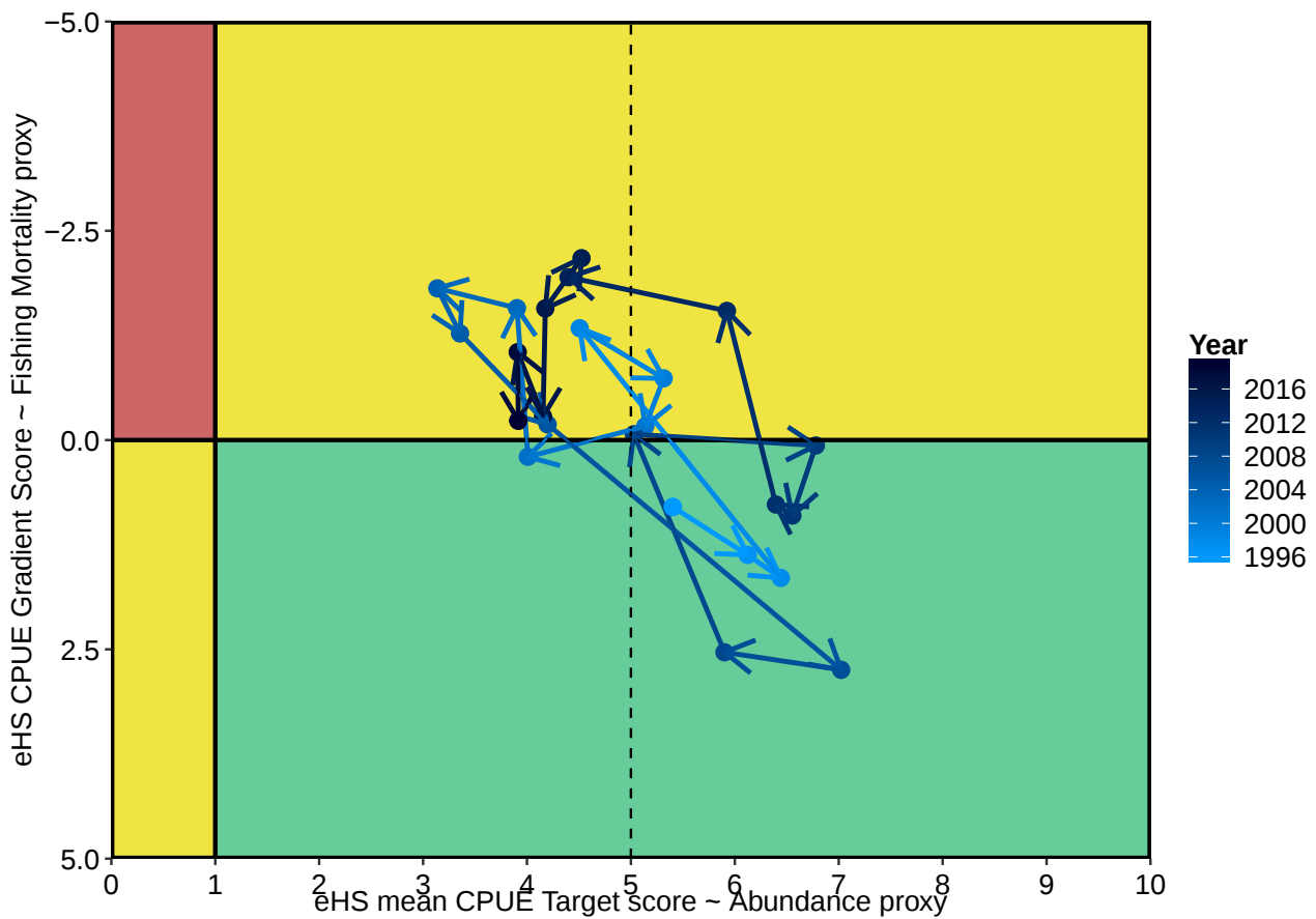
Figure 3.76: Phase plot of fishing mortality and abundance proxies for greenlip abalone, 1996–2019. The Gradient 4 PM (y-axis) is used as a proxy for fishing mortality, and the Target CPUE PM is used as a proxy for abundance. Zone score is calculated as a catch-weighted mean of individual regional scores.
