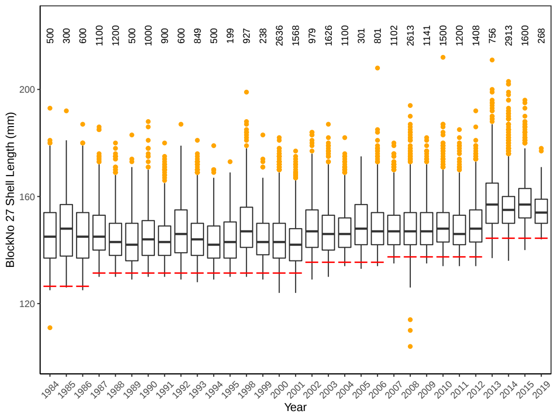
Figure 3.95: Boxplot of size distributions for Block 27 Eastern Zone between 1984 and 2019. Red line indicates legal minimum length for that year. Number of abalone measured given above each boxplot.
