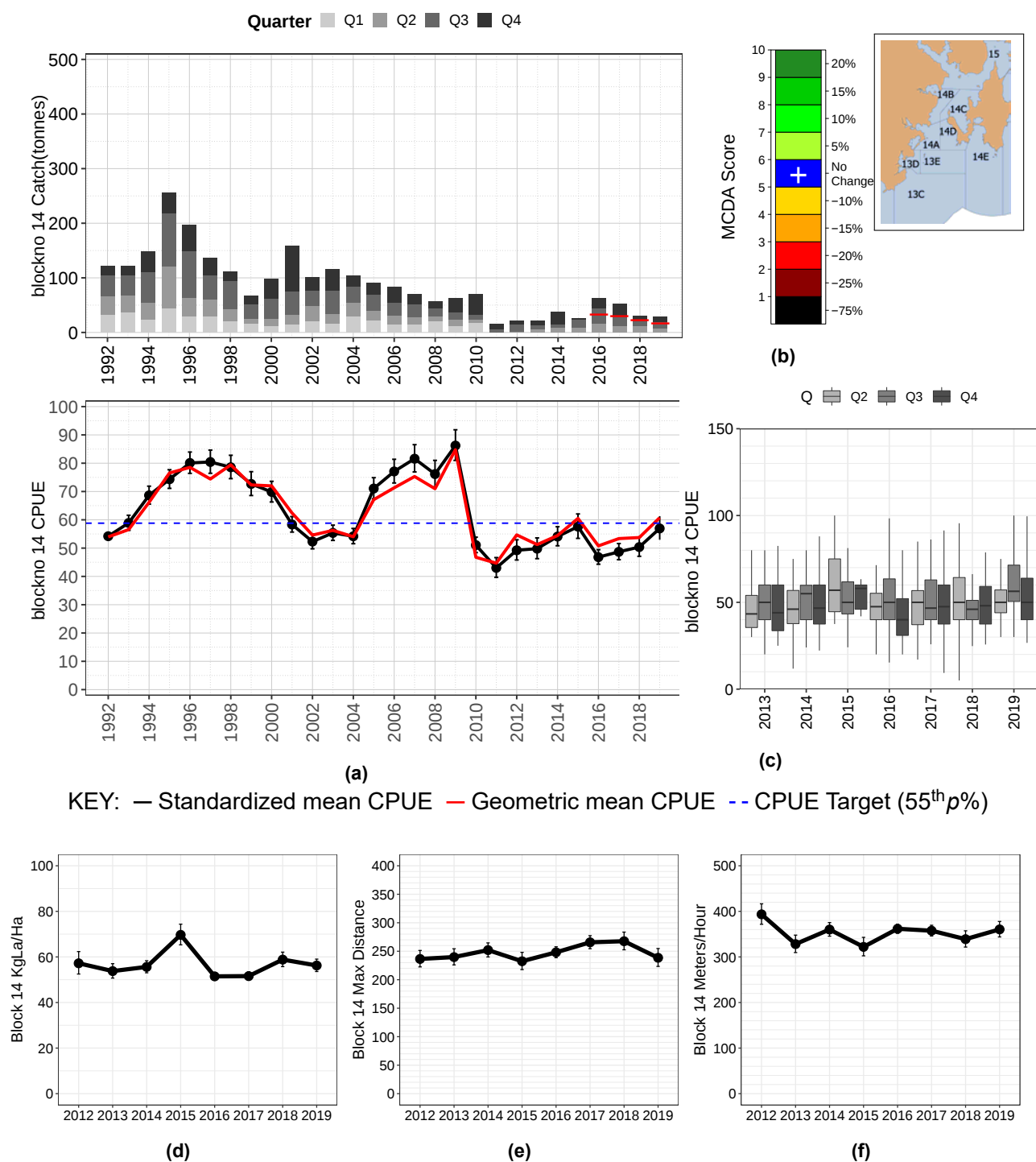
Figure 3.8: Block 14 EZ: a) Catch per quarter (bars) standardised CPUE (black with SE bars) and unstandardised CPUE (red); b) HCR outcome; c) CPUE boxplot by quarter; d) mean KgLa/Ha based on dive vessel footprint from kernel density analysis; e) mean maximum length of dive; f) mean swim rate in metres of coast per hour. Note: all means are bias corrected geometric means.
