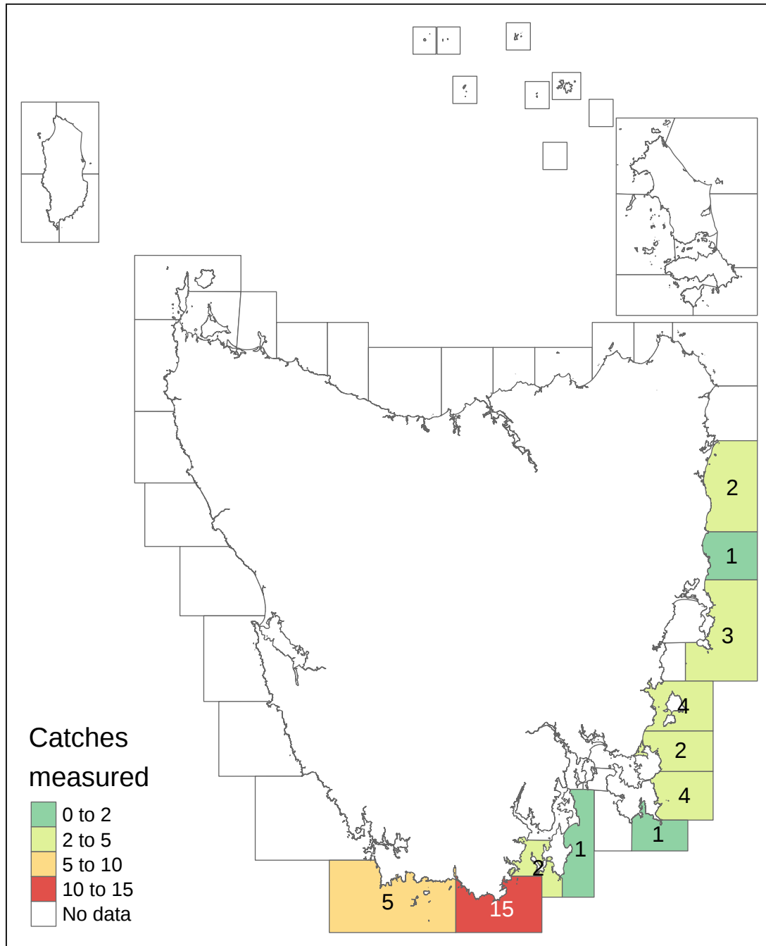
Figure 3.85: Distribution and number of commercial abalone catches sampled for length-frequency data across reporting Blocks during 2019.
