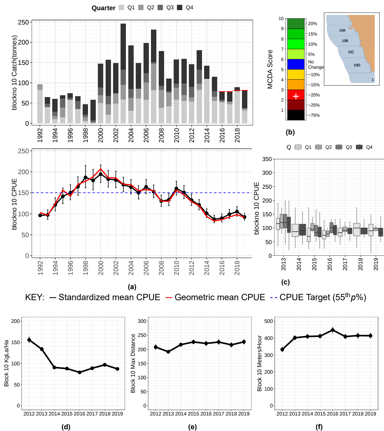
Figure 3.32: Block 10 WZ: a) Catch per quarter (bars) standardised CPUE (black with SE bars) and un-standardised CPUE (red); b) HCR outcome; c) CPUE boxplot by quarter; d) mean KgLa/Ha based on dive vessel footprint from kernel density analysis; e) mean maximum length of dive; f) mean swim rate in metres of coast per hour. Note: all means are bias corrected geometric means.
