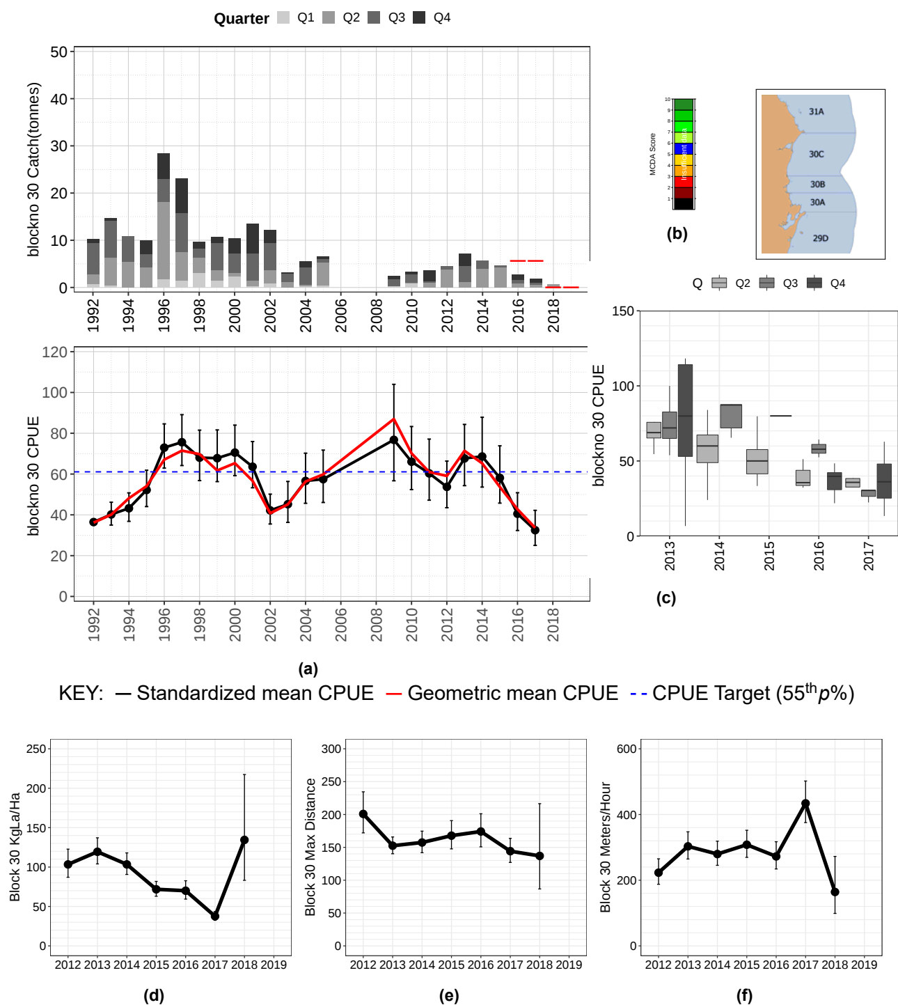
Figure 3.20: Block 30 EZ: a) Catch per quarter (bars) standardised CPUE (black with SE bars) and un-standardised CPUE (red); b) HCR outcome; c) CPUE boxplot by quarter; d) mean KgLa/Ha based on dive vessel footprint from kernel density analysis; e) mean maximum length of dive; f) mean swim rate in metres of coast per hour. Note: all means are bias corrected geometric means.
