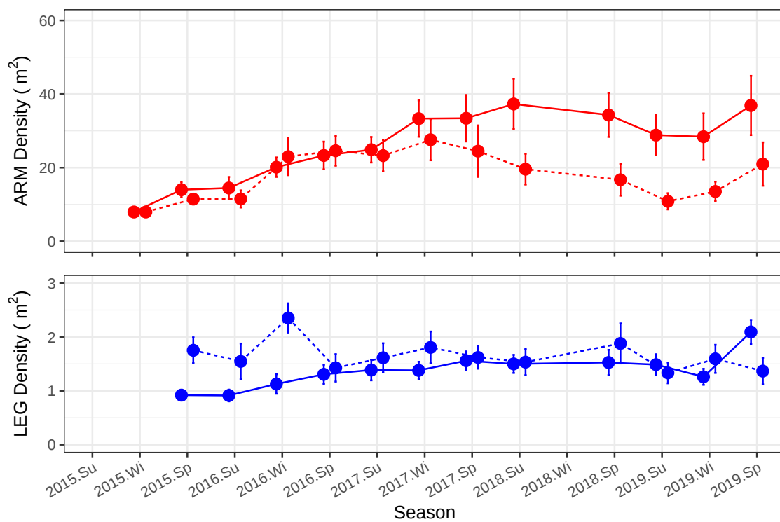
Figure 4.1: Mean density ( m^2 ) of abalone ( \pm SE) underneath ARMs (red) and recorded from LEG (blue) across the sampling period Summer 2015 to Spring 2019 at Black Reef boulder site (Block 14A). Each ARM has a planar surface area of 0.126m^2 . Replicate strings (sub-sites) are denoted by line type. Note the difference in density scale between the ARM and LEG results.
