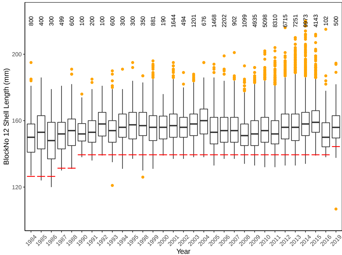
Figure 3.87: Boxplot of size distributions for Block 12 Western Zone between 1984 and 2019. Red line indicates legal minimum length for that year. Number of abalone measured given above each boxplot.
