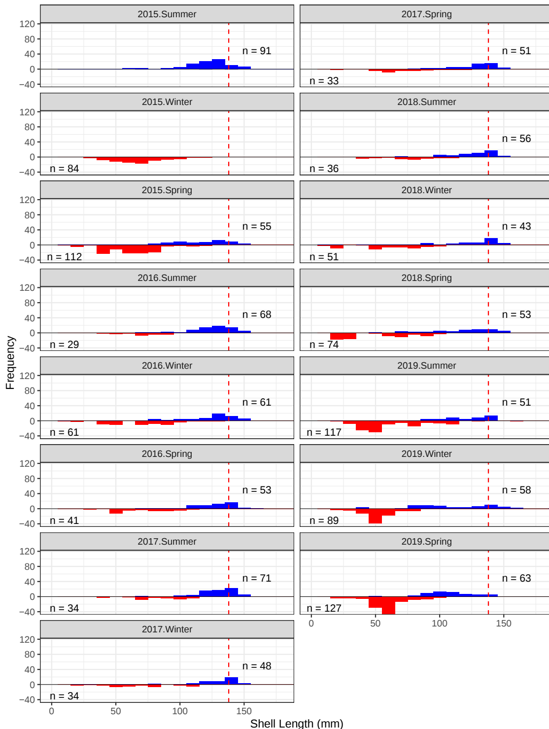
Figure 4.8: Size frequency of abalone recorded underneath ARMs (red) and from LEG (blue) across the sampling period Summer 2015 to Spring 2019 at Betsey Island (Block 17A). Hashed red line represents the LML for that year. Total number of abalone measured for ARMs (lower) and LEG (upper) during each sampling period are also given.
