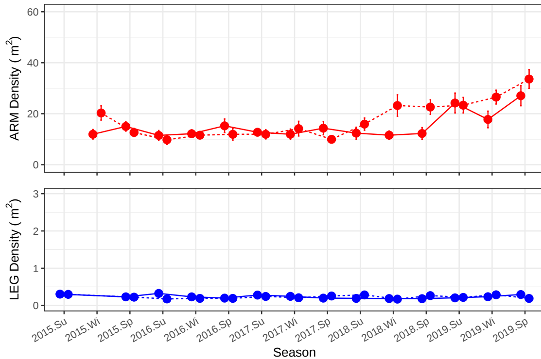
Figure 4.7: Mean density ( m^2 ) of abalone (+/- SE) underneath ARMs (red) and recorded from LEG (blue) across the sampling period Summer 2015 to Spring 2019 at Betsey Island (Block 17A). Each ARM has a planar surface area of 0.126m^2 . Replicate strings (sub-sites) are denoted by line type. Note the difference in density scale between the ARM and LEG results.
