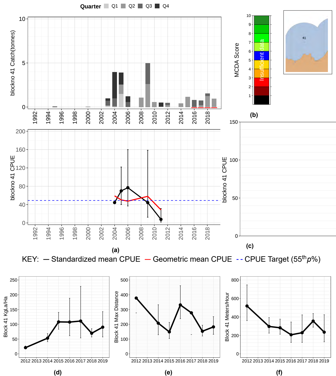
Figure 3.67: Block 41 BSZ: a) Catch per quarter (bars) standardised CPUE (black with SE bars) and unstandardised CPUE (red); b) HCR outcome; c) CPUE boxplot by quarter; d) mean KgLa/Ha based on dive vessel footprint from kernel density analysis; e) mean maximum length of dive; f) mean swim rate in metres of coast per hour. Note: all means are bias corrected geometric means.
