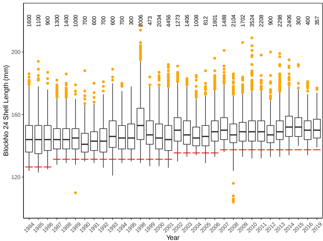
Figure 3.94: Boxplot of size distributions for Block 24 Eastern Zone between 1984 and 2019. Red line indicates legal minimum length for that year. Number of abalone measured given above each boxplot.
