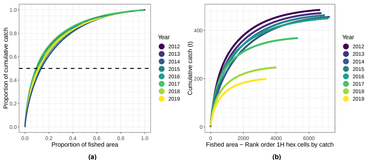
Figure 3.5: Concentration area curves for catch in the Eastern Zone: a) Proportion of catch (y axis) against proportion of reef utilised (x axis). Hashed line represents 50% of catch; b) cumulative catch (y axis) against rank order of hex cells, descending from highest to smallest catch. Data filtered to exclude hex cells where less than 5 minutes of effort observed.
