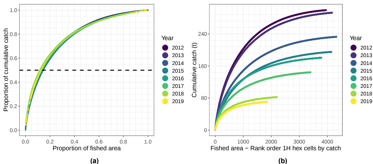
Figure 3.44: Concentration area curves for catch in the Northern Zone: a) Proportion of catch (y axis) against proportion of reef utilised (x axis). Hashed line represents 50% of catch; b) cumulative catch (y axis) against rank order of hex cells, descending from highest to smallest catch. Data filtered to exclude hex cells where less than 5 minutes of effort observed.
