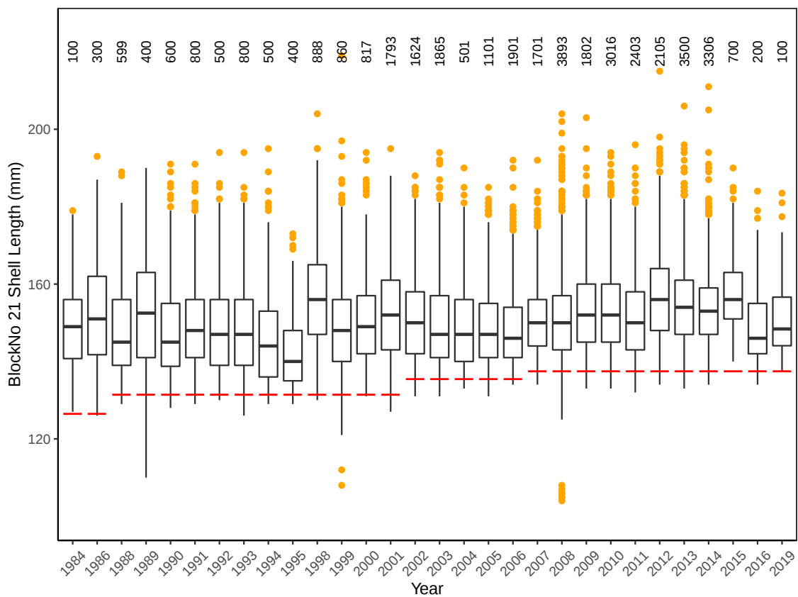
Figure 3.91: Boxplot of size distributions for Block 21 Eastern Zone between 1984 and 2019. Red line indicates legal minimum length for that year. Number of abalone measured given above each boxplot.
