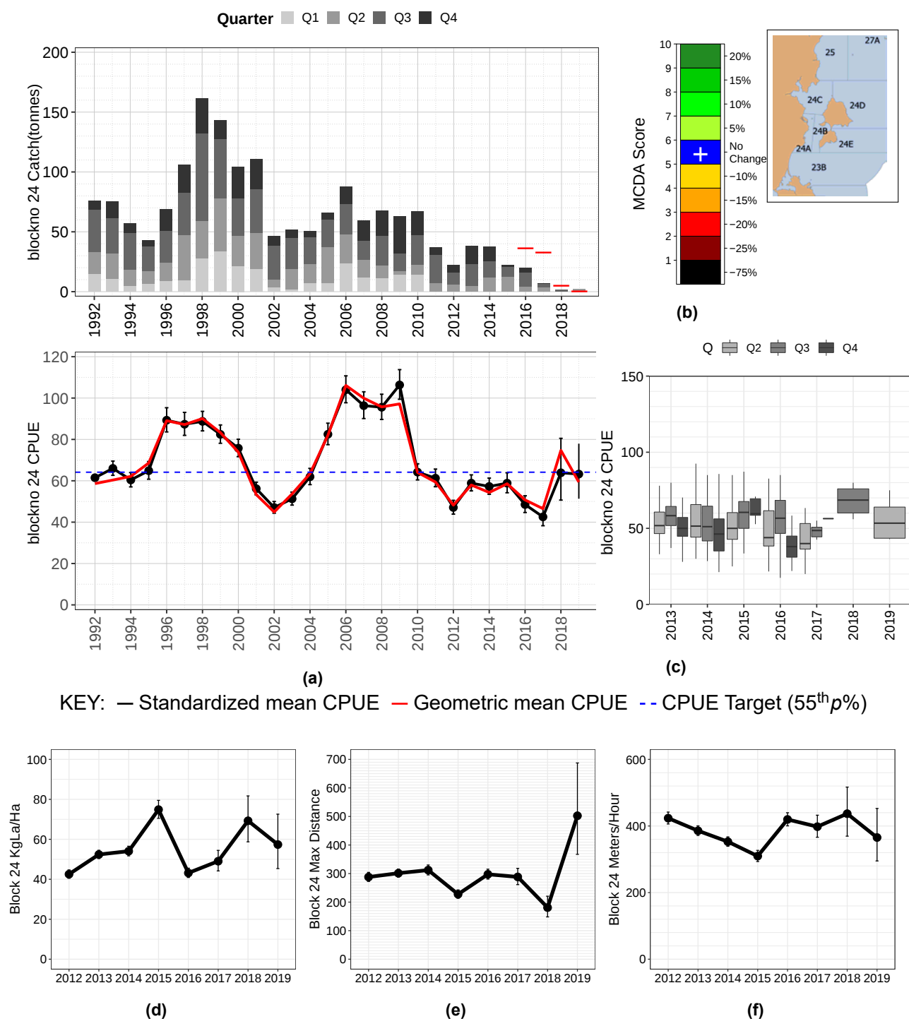
Figure 3.16: Block 24 EZ: a) Catch per quarter (bars) standardised CPUE (black with SE bars) and un-standardised CPUE (red); b) HCR outcome; c) CPUE boxplot by quarter; d) mean KgLa/Ha based on dive vessel footprint from kernel density analysis; e) mean maximum length of dive; f) mean swim rate in metres of coast per hour. Note: all means are bias corrected geometric means.
