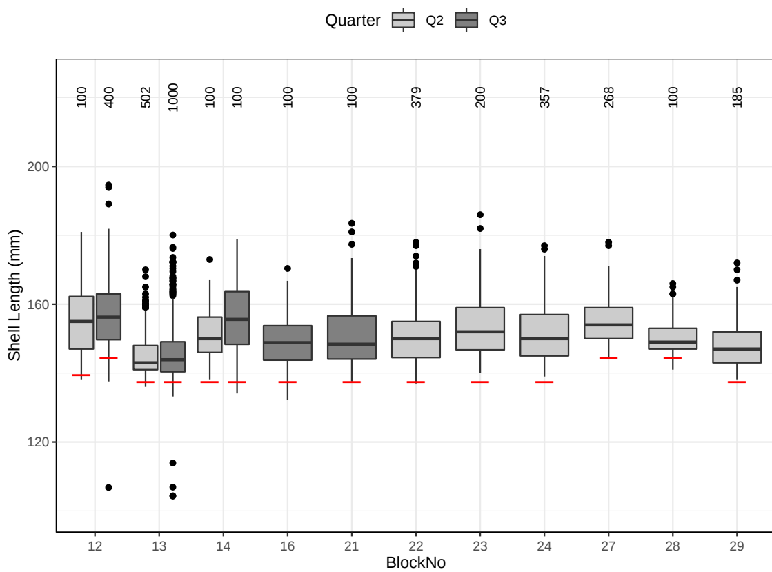
Figure 3.86: Boxplot of catch size distribution by reporting Block and quarter catches sampled in 2019. Red line indicates legal minimum length. Number of abalone measured given above each boxplot.
