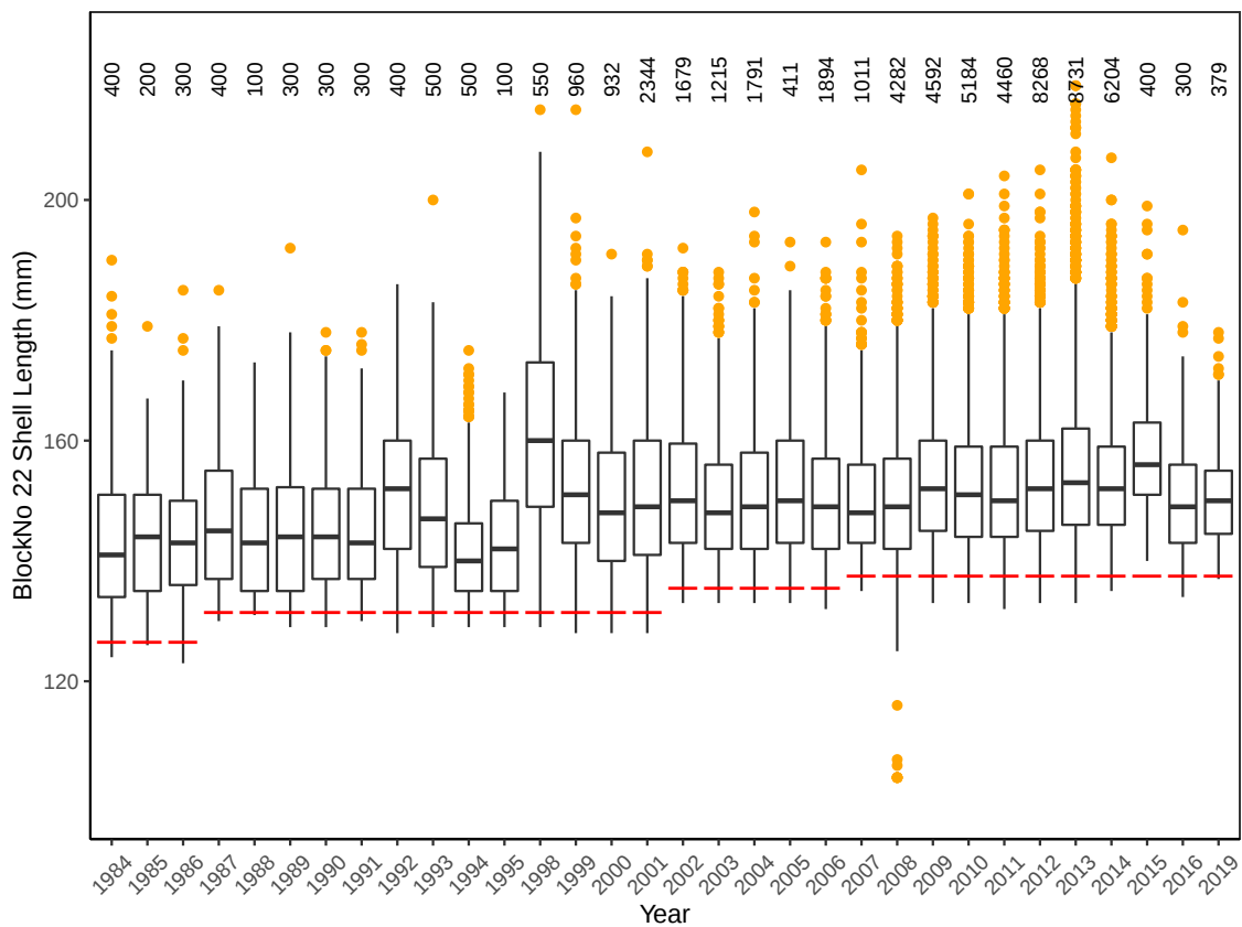
Figure 3.92: Boxplot of size distributions for Block 22 Eastern Zone between 1984 and 2019. Red line indicates legal minimum length for that year. Number of abalone measured given above each boxplot.
