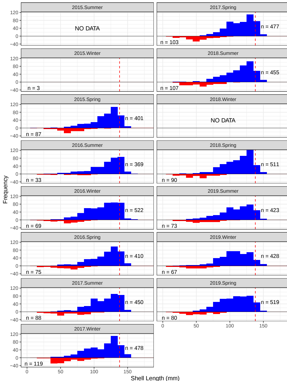
Figure 4.2: Size frequency of abalone recorded underneath ARMs (red) and from LEG (blue) across the sampling period Summer 2015 to Spring 2019 at Black Reef Boulder (Block 14A). Hashed red line represents the LML for that year. Total number of abalone measured for ARMs (lower) and LEG (upper) during each sampling period are also given.
