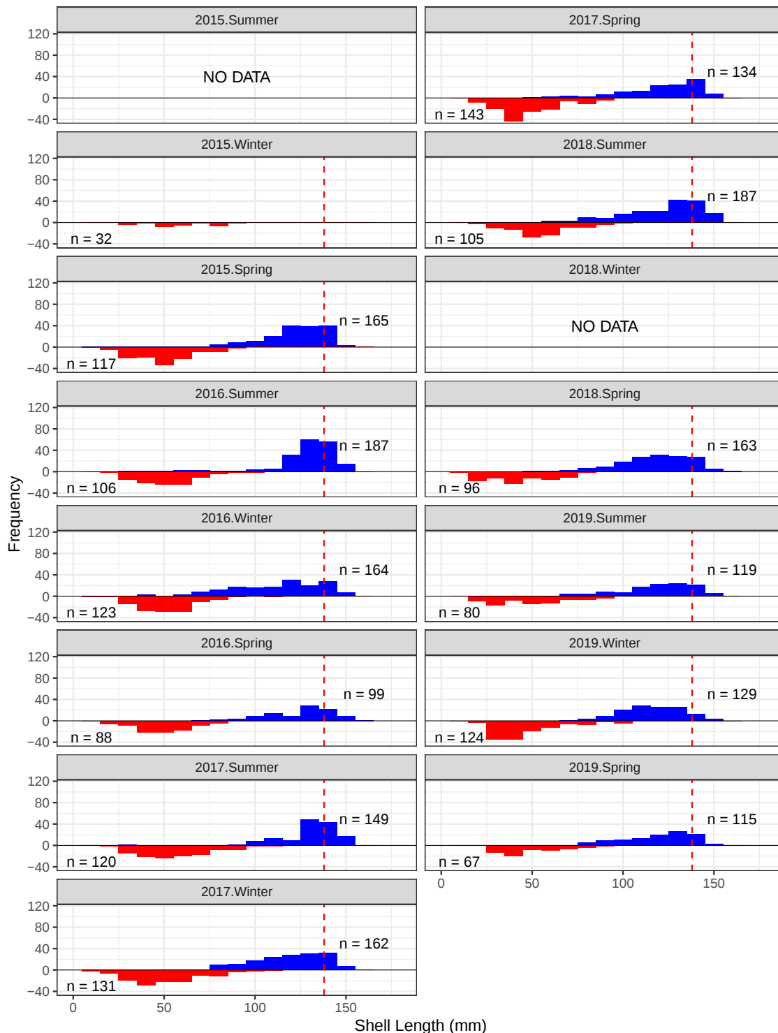
Figure 4.6: Size frequency of abalone recorded underneath ARMs (red) and from LEG (blue) across the sampling period Summer 2015 to Spring 2019 at George III Rock. Hashed red line represents the LML for that year. Total number of abalone measured for ARMs (lower) and LEG (upper) during each sampling period are also given.
