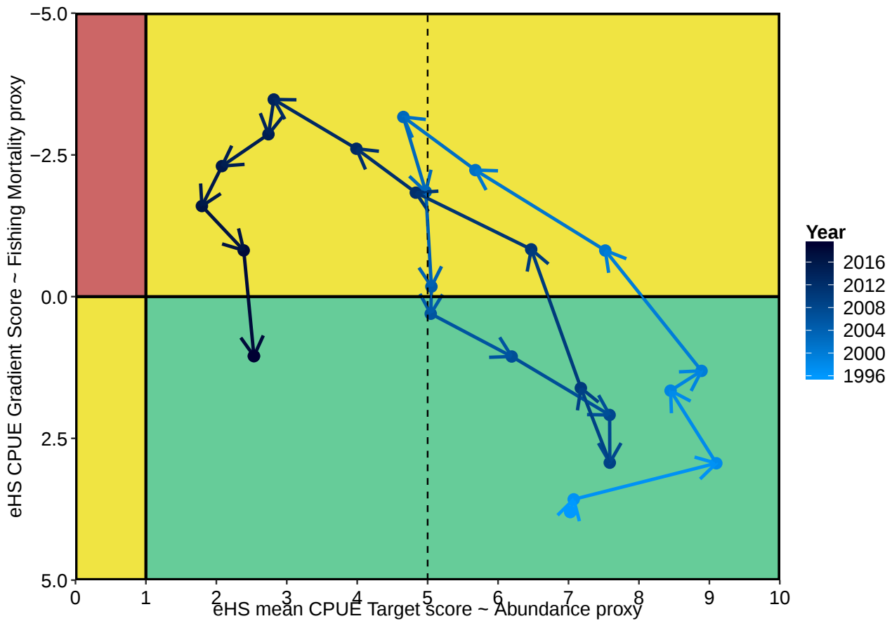
Figure 3.43: Phase plot of fishing mortality and abundance proxies for Northern Zone blacklip abalone , 1996–2019. The Gradient 4 PM (y-axis) is used as a proxy for fishing mortality, and the Target CPUE PM is used as a proxy for abundance. Zone score is calculated as a catch-weighted mean of individual block scores.
