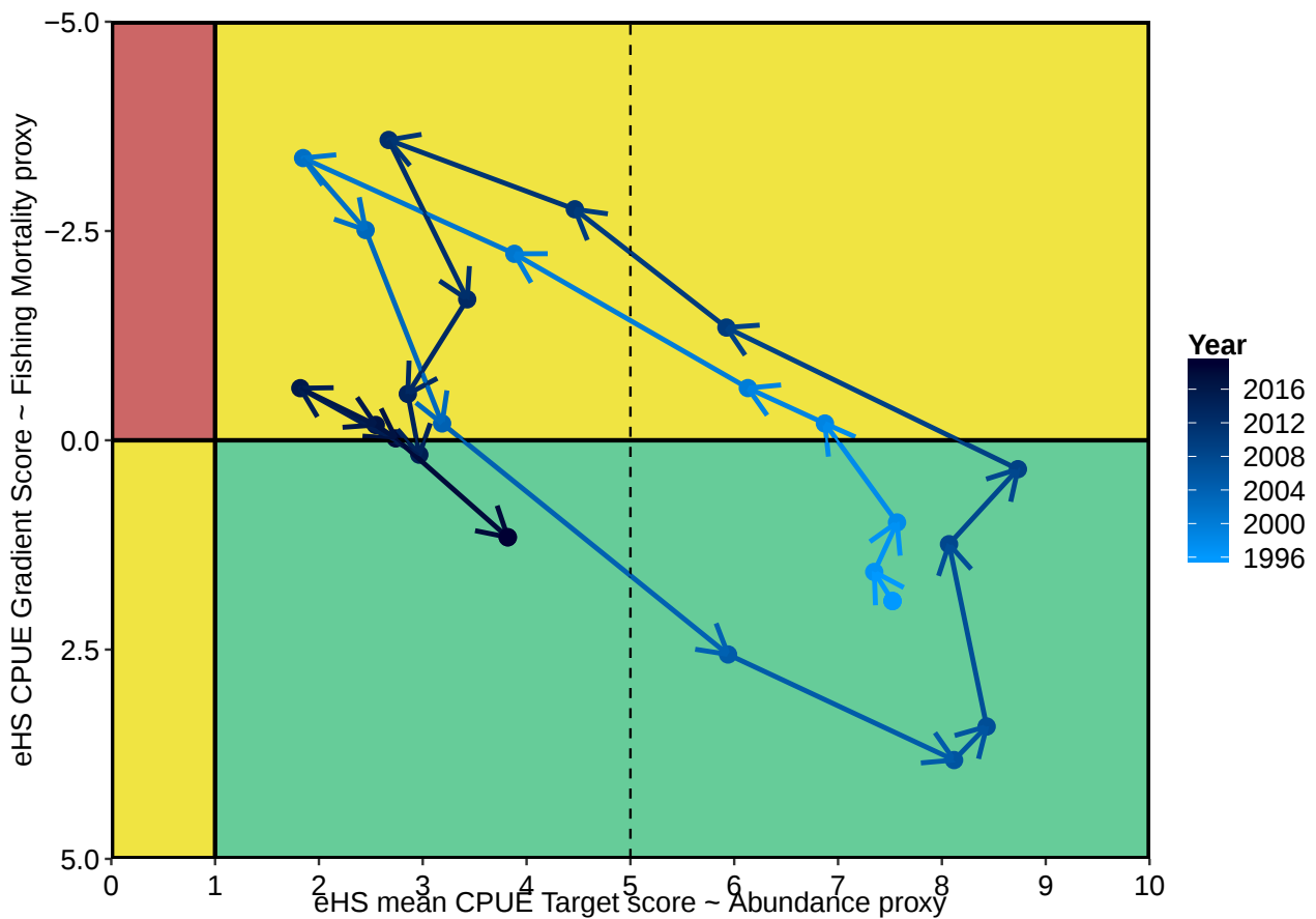
Figure 3.4: Phase plot of fishing mortality and abundance proxies for Eastern Zone blacklip abalone , 1996–2019. The Gradient 4 PM (y-axis) is used as a proxy for fishing mortality, and the Target CPUE PM is used as a proxy for abundance. Zone score is calculated as a catch-weighted mean of individual block scores.
