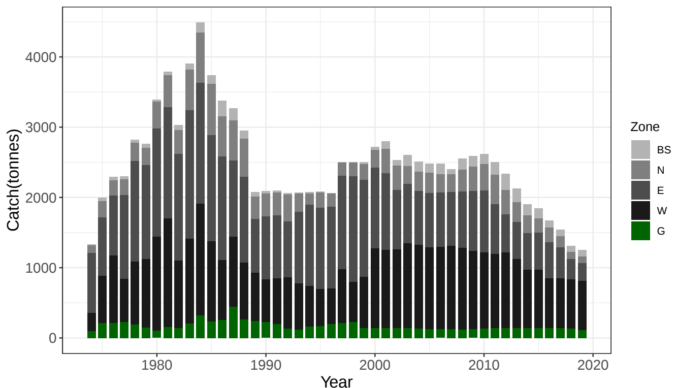
Figure 1.1: Annual blacklip abalone ( Haliotis rubra ) and greenlip abalone ( H. laevisgata ) from 1974 to 2019. Bars colour coded by current zonation system.
