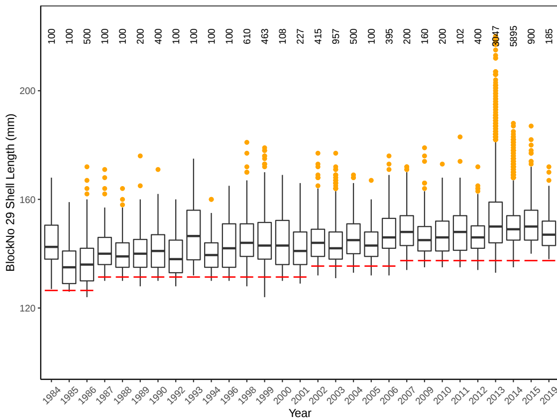
Figure 3.97: Boxplot of size distributions for Block 29 Eastern Zone between 1984 and 2019. Red line indicates legal minimum length for that year. Number of abalone measured given above each boxplot.
