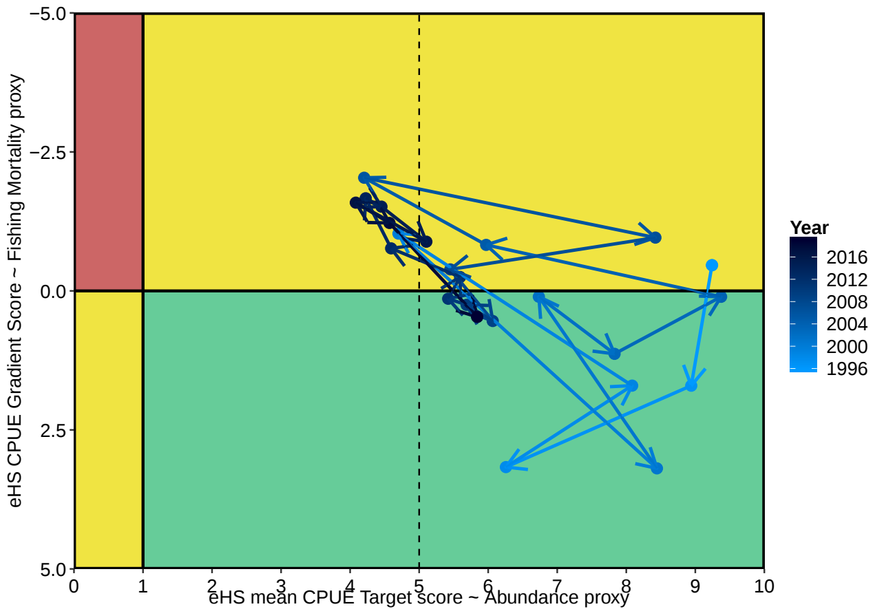
Figure 3.58: Phase plot of fishing mortality and abundance proxies for Bass Strait Zone blacklip abalone , 1996–2019. The Gradient 4 PM (y-axis) is used as a proxy for fishing mortality, and the Target CPUE PM is used as a proxy for abundance. Zone score is calculated as a catch-weighted mean of individual block scores.
