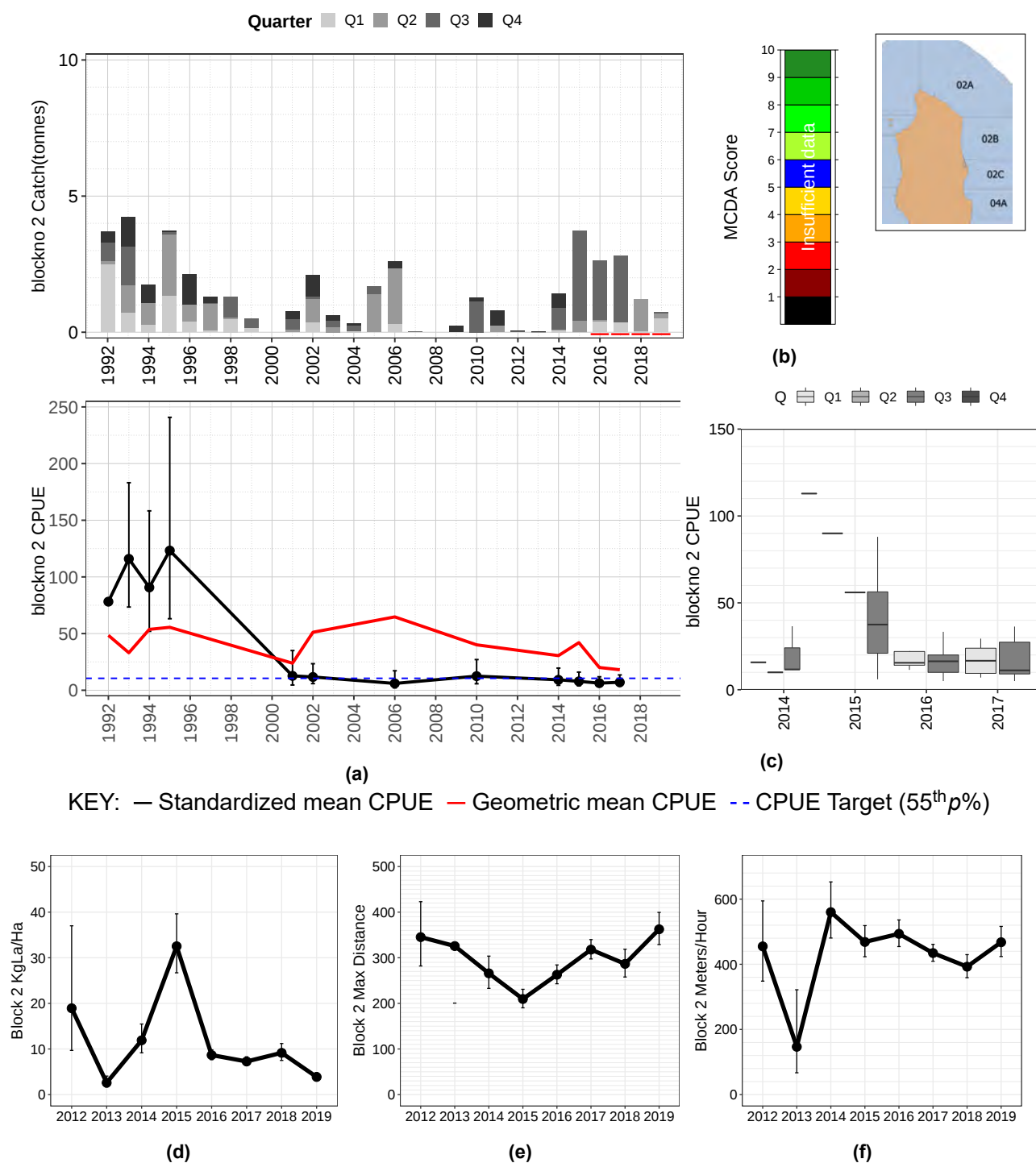
Figure 3.52: Block 2 NZ: a) Catch per quarter (bars) standardised CPUE (black with SE bars) and unstandardised CPUE (red); b) HCR outcome; c) CPUE boxplot by quarter; d) mean KgLa/Ha based on dive vessel footprint from kernel density analysis; e) mean maximum length of dive; f) mean swim rate in metres of coast per hour. Note: all means are bias corrected geometric means.
