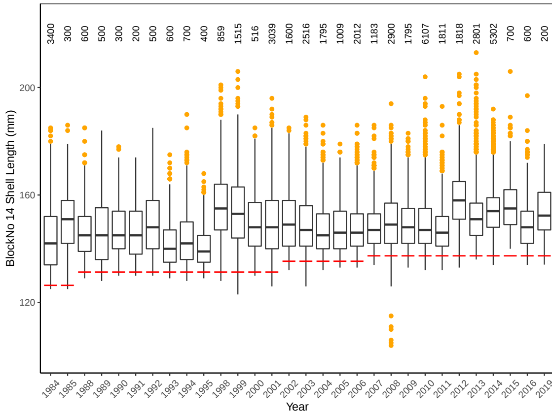
Figure 3.89: Boxplot of size distributions for Block 14 Eastern Zone between 1984 and 2019. Red line indicates legal minimum length for that year. Number of abalone measured given above each boxplot.
