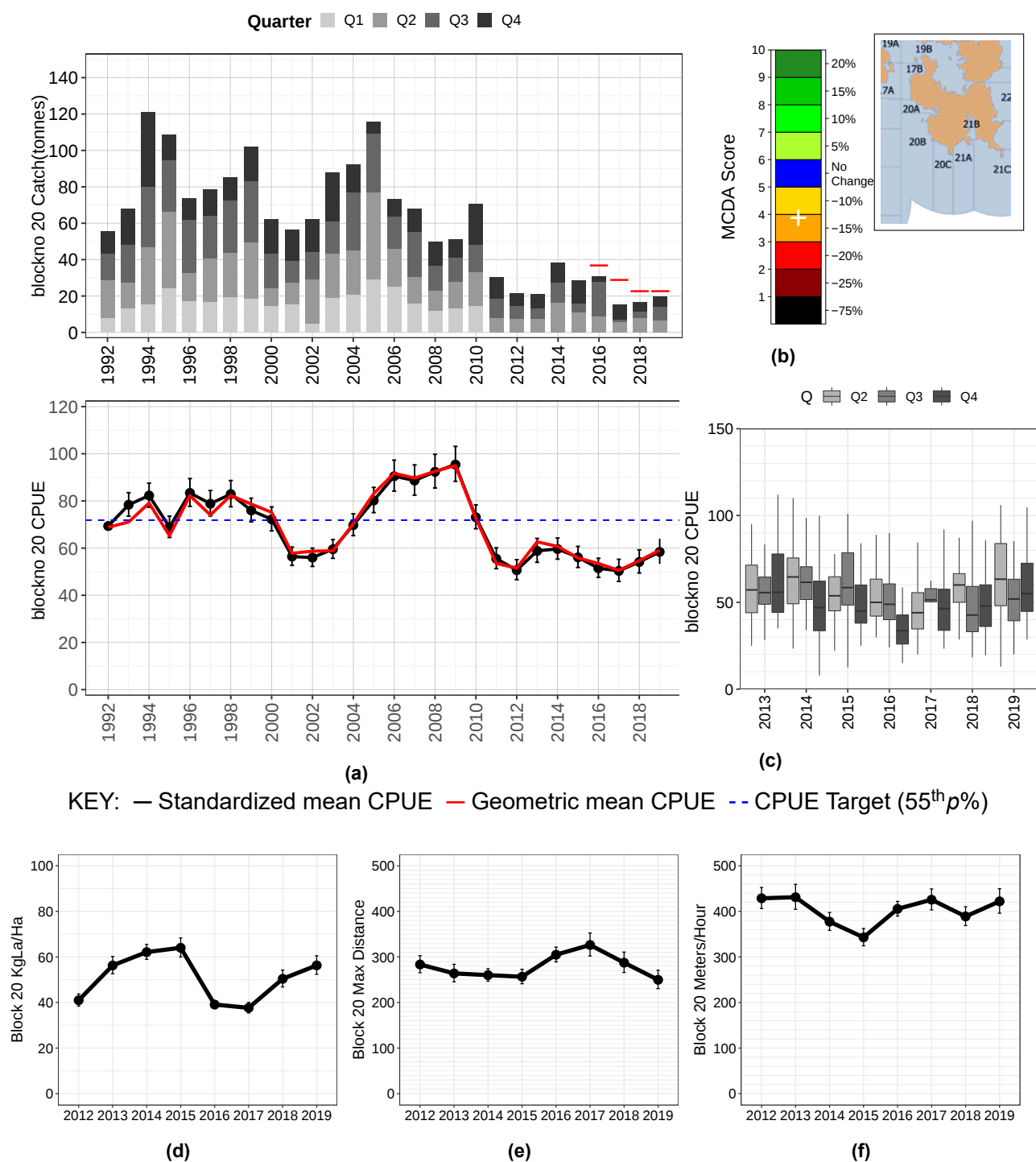
Figure 3.12: Block 20 EZ: a) Catch per quarter (bars) standardised CPUE (black with SE bars) and un-standardised CPUE (red); b) HCR outcome; c) CPUE boxplot by quarter; d) mean KgLa/Ha based on dive vessel footprint from kernel density analysis; e) mean maximum length of dive; f) mean swim rate in metres of coast per hour. Note: all means are bias corrected geometric means.
