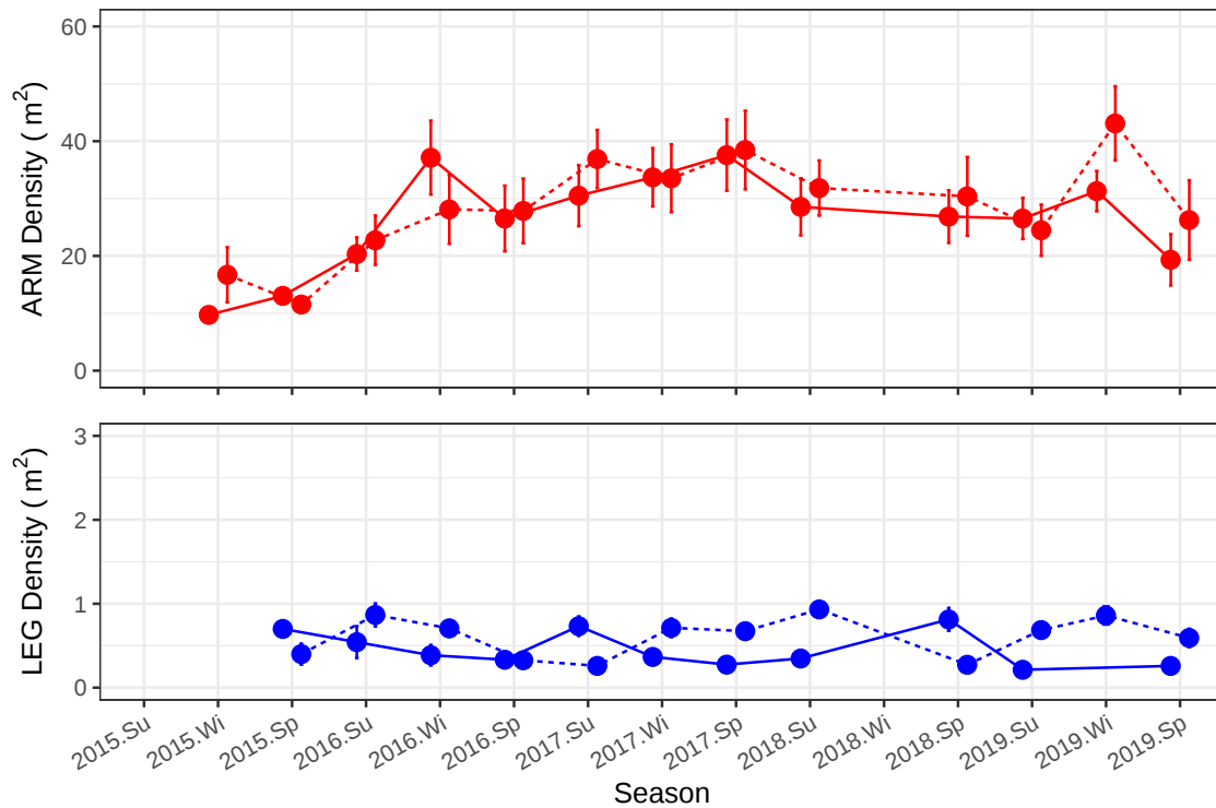
Figure 4.5: Mean density (m 2 ) of abalone (+/- SE) underneath ARMs (red) and recorded from LEG (blue) across the sampling period Summer 2015 to Spring 2019 at George III Rock. Each ARM has a planar surface area of 0.126m 2 . Replicate strings (sub-sites) are denoted by line type. Note the difference in density scale between the ARM and LEG results.
